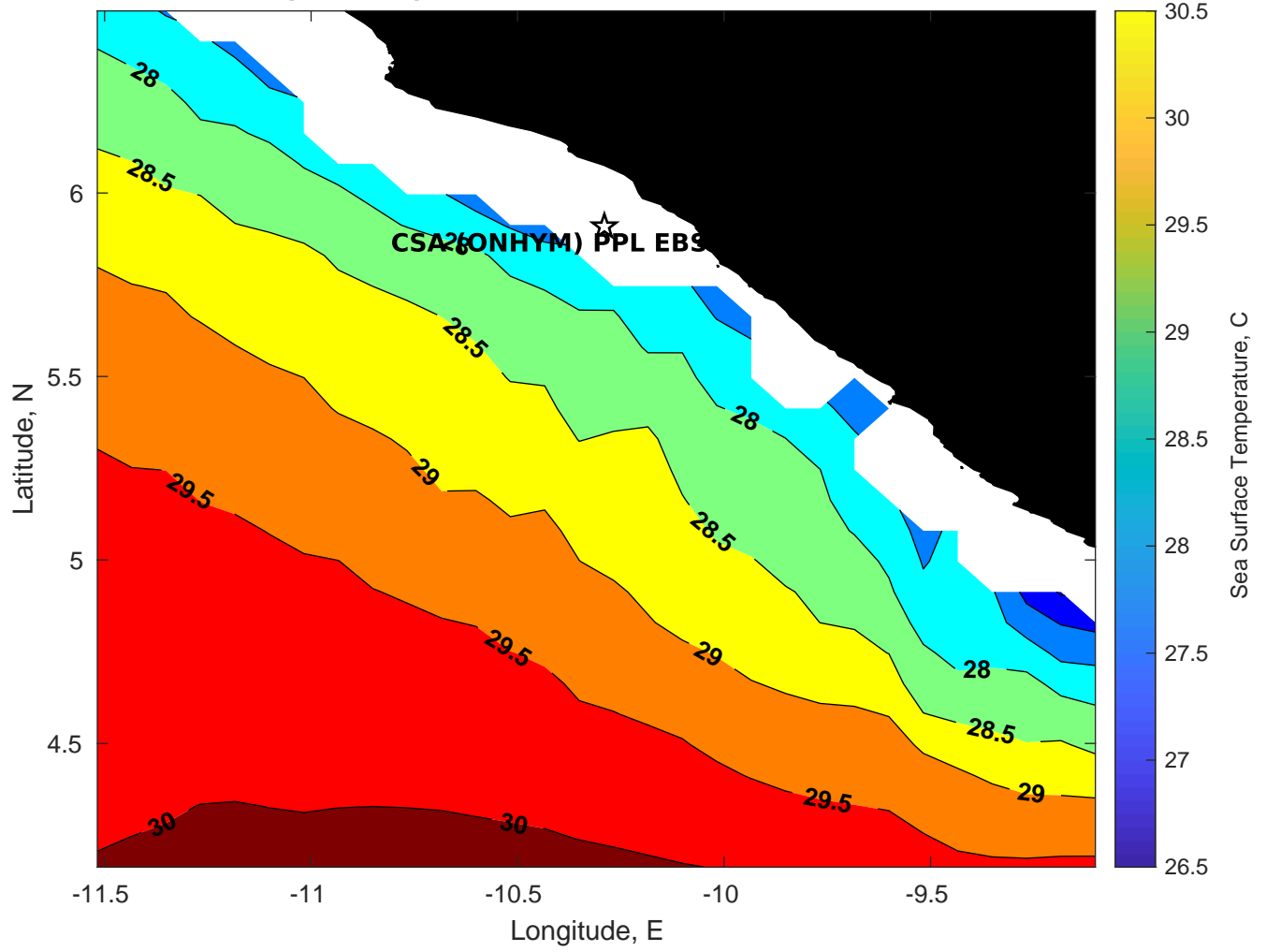
SST for CSA (ONHYM) PPL EBS - Liberia at 28-Feb-2025 00:00:00
