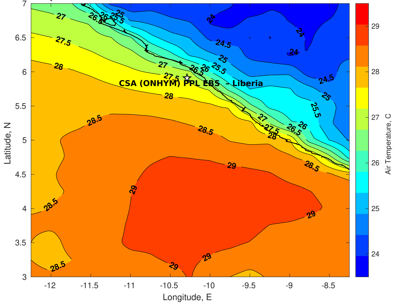
Air Temperature (C) for CSA (ONHYM) PPL EBS - Liberia at 01-Mar-2025
