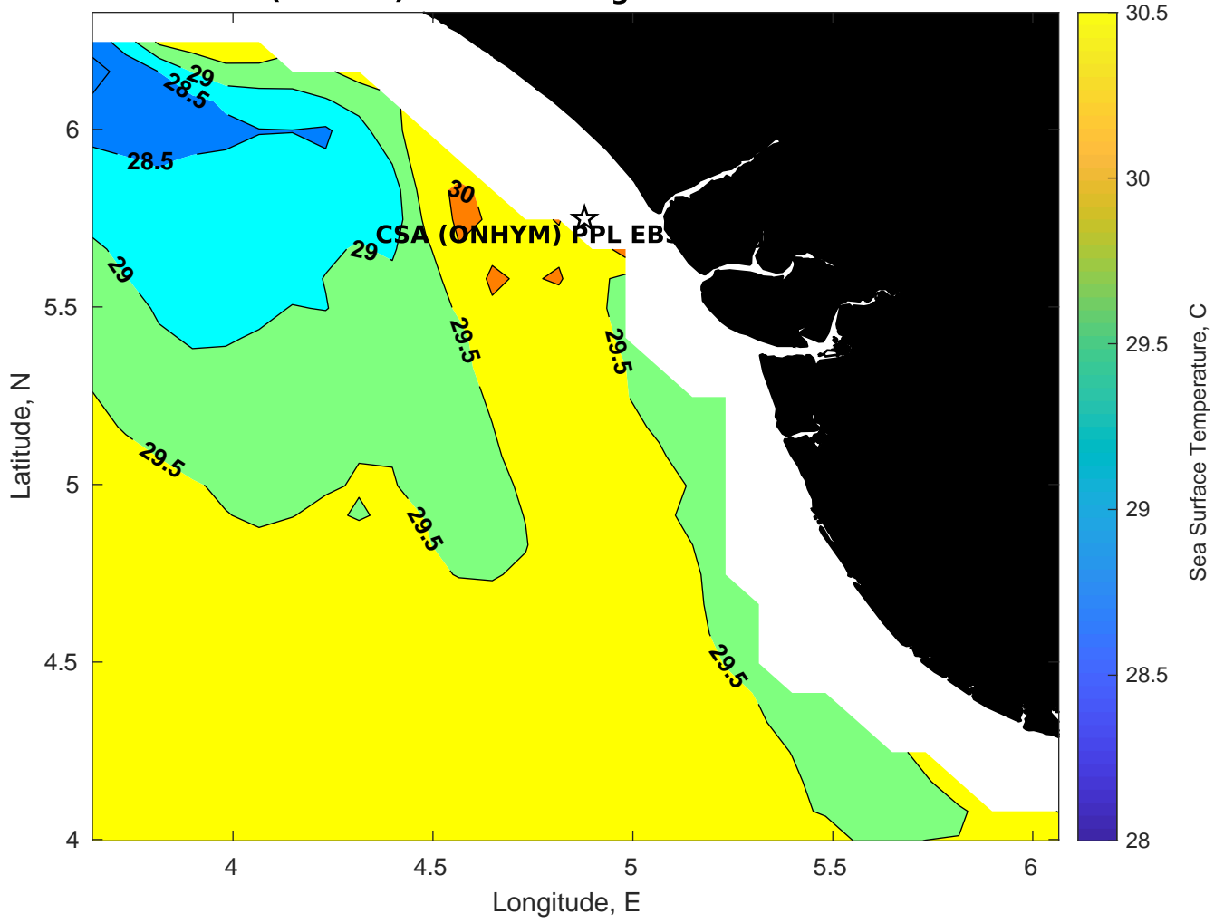
SST for CSA (ONHYM) PPL EBS - Nigeria at 28-Feb-2025 00:00:00
