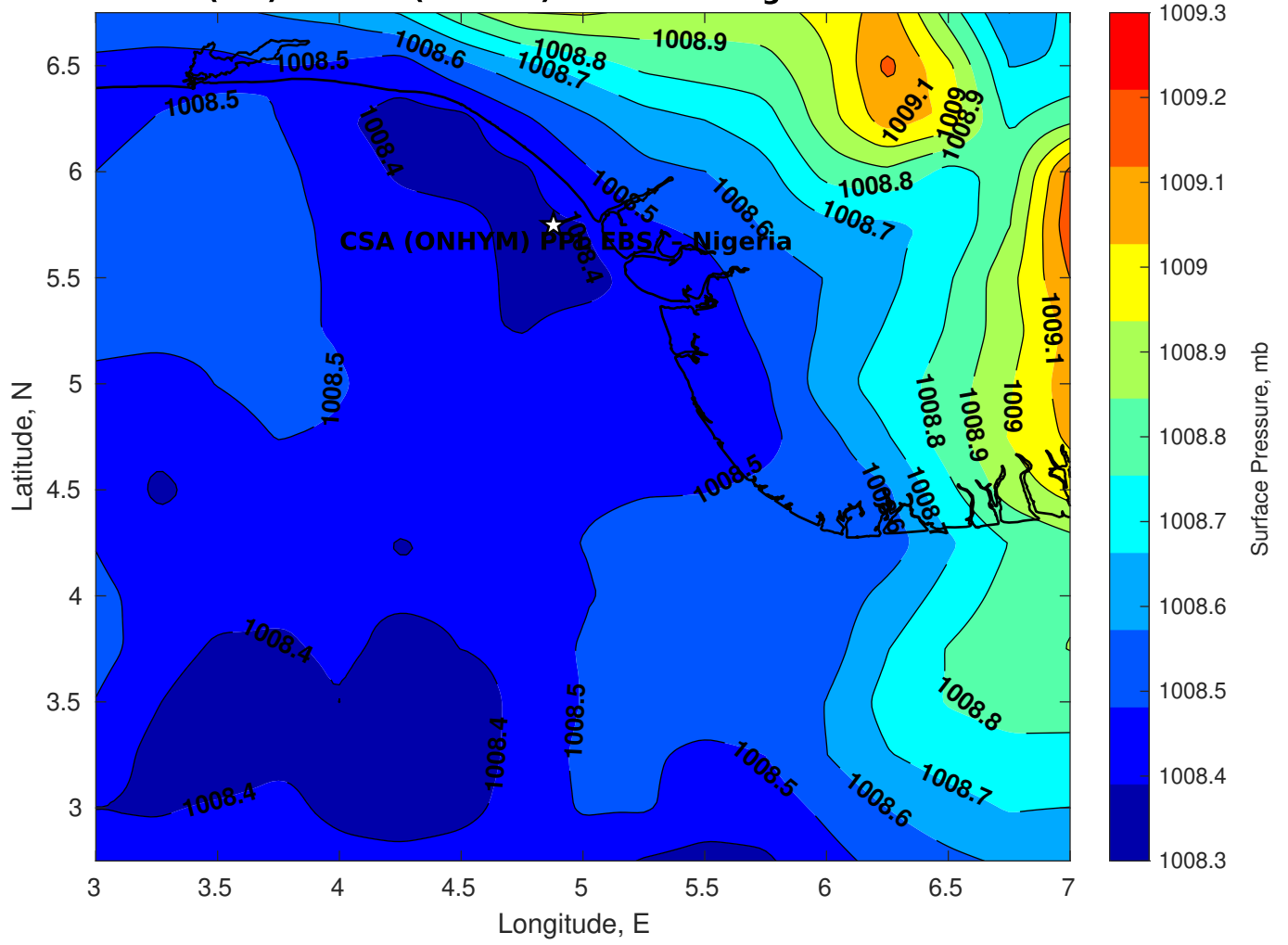
Surface Pressure (mb) for CSA (ONHYM) PPL EBS - Nigeria at 02-Mar-2025 06:00:00
