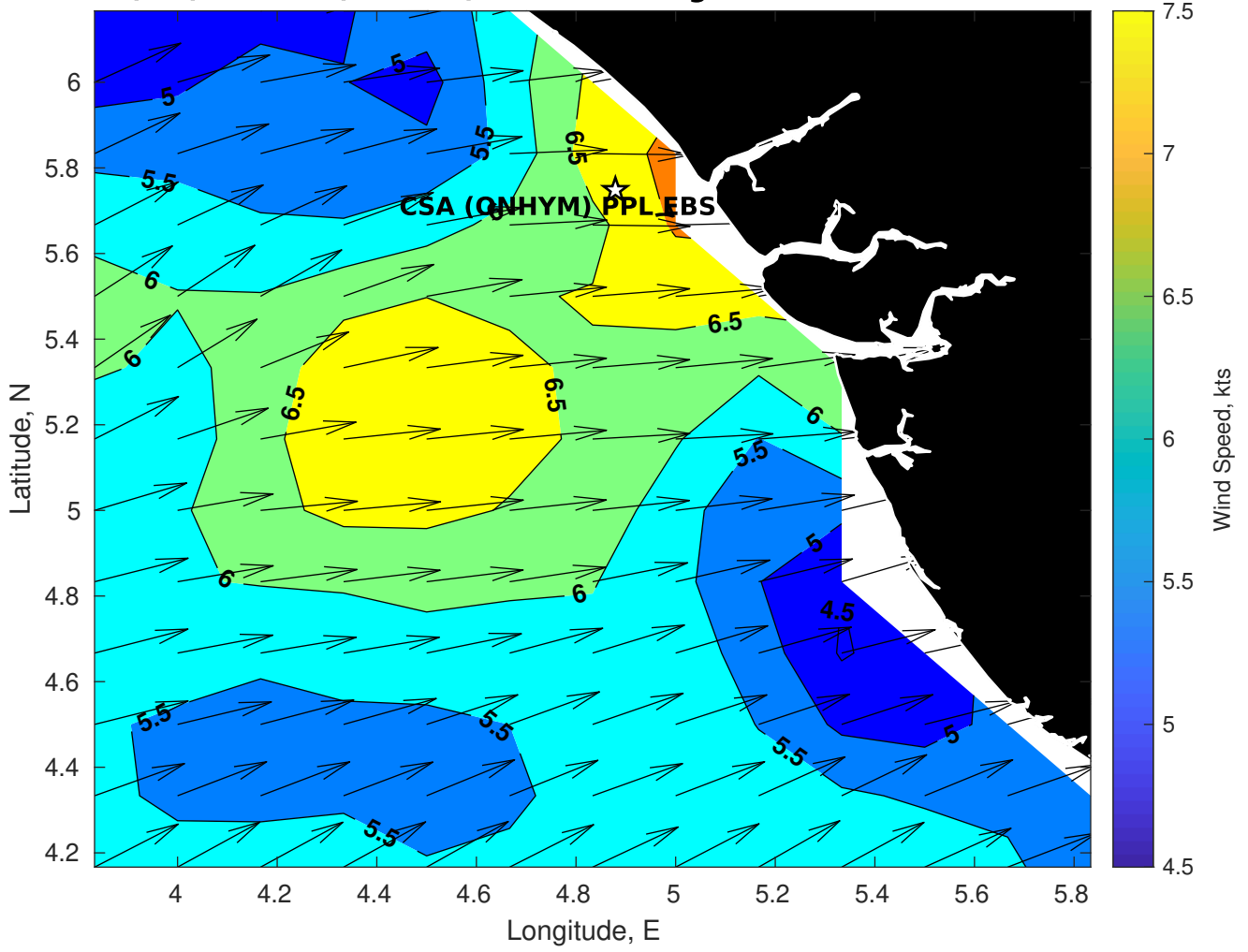
Winds (kts) for CSA (ONHYM) PPL EBS - Nigeria at 01-Mar-2025 09:00:00
