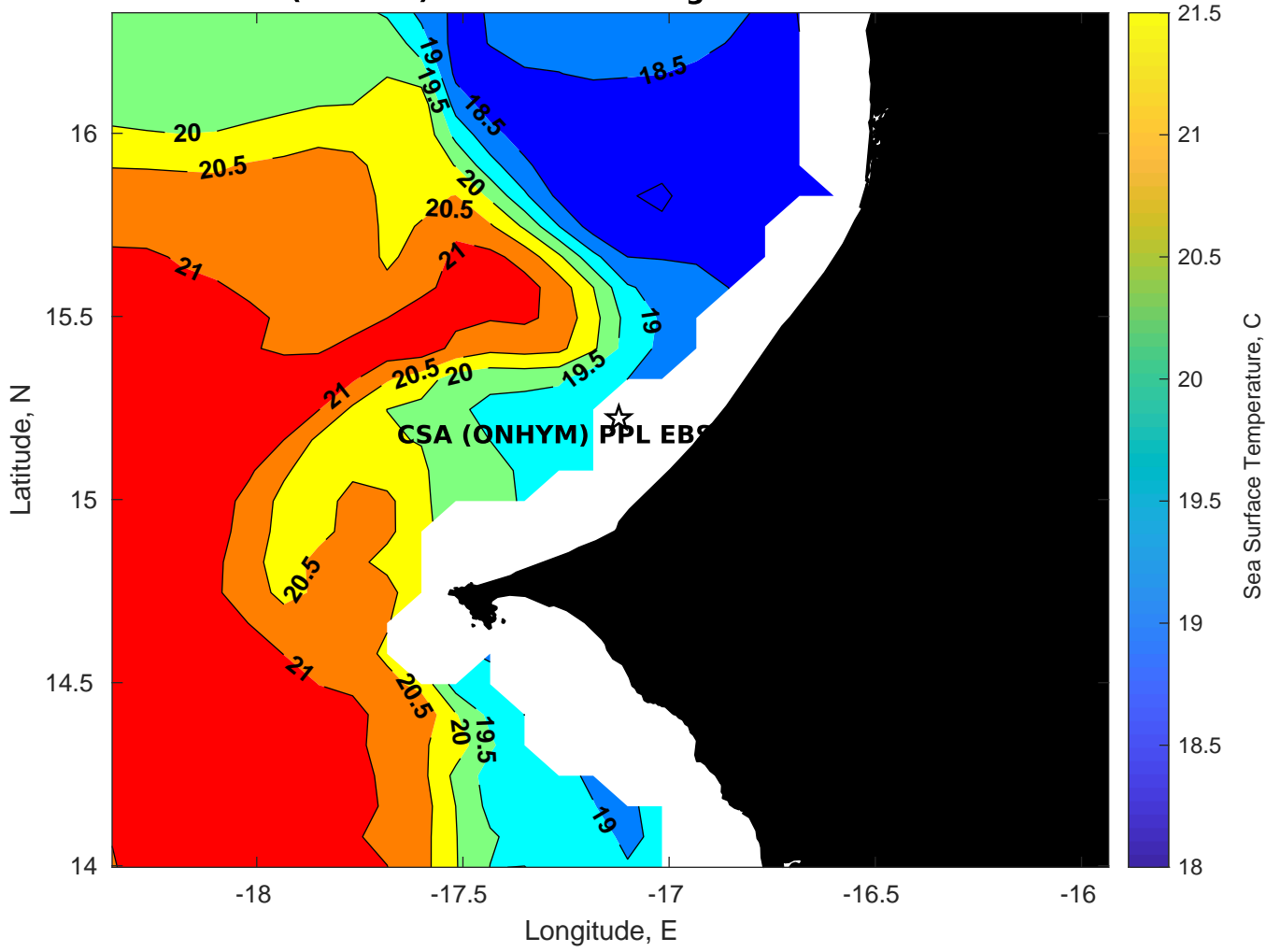
SST for CSA (ONHYM) PPL EBS - Senegal at 28-Feb-2025 00:00:00
