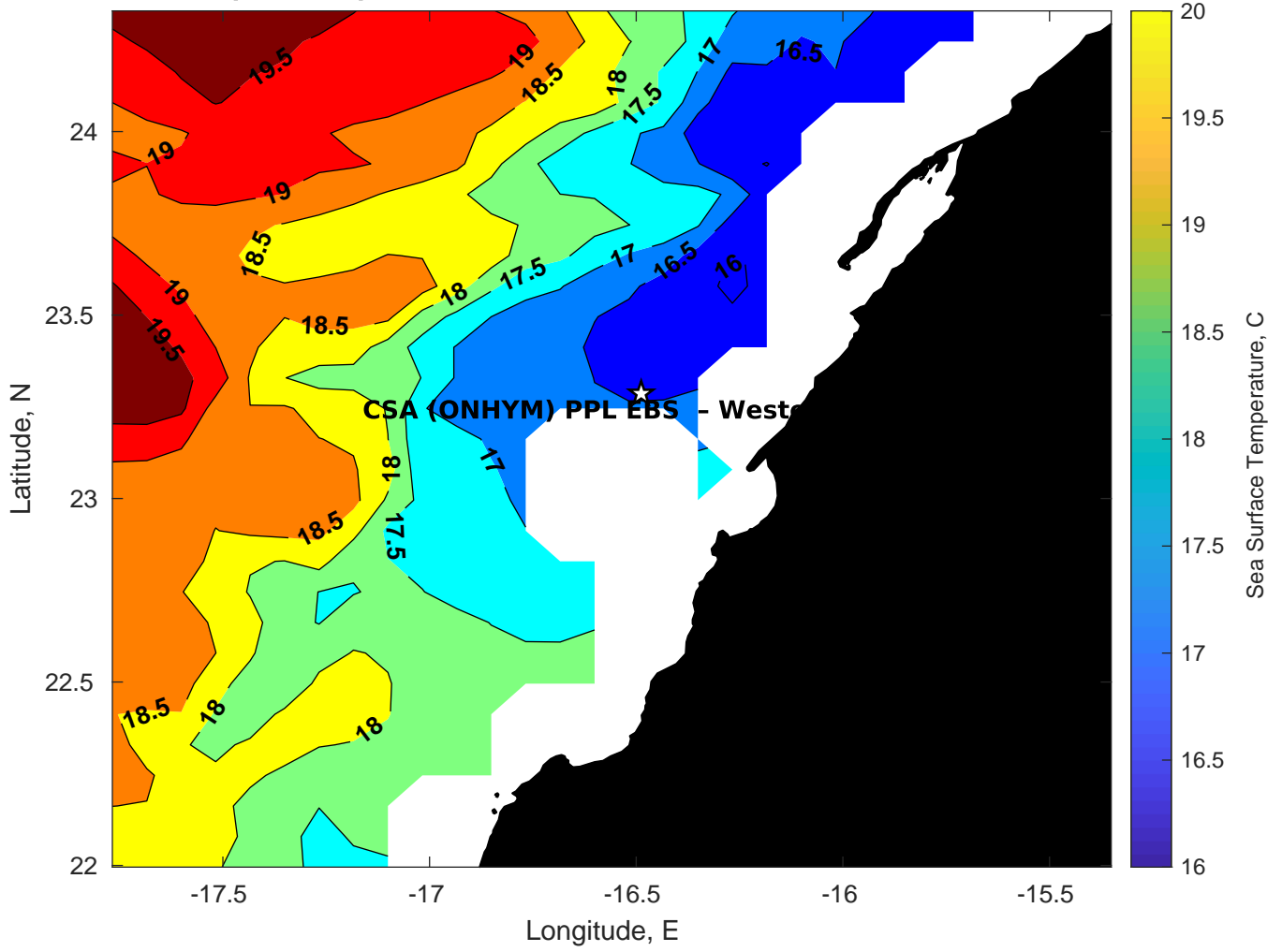
SST for CSA (ONHYM) PPL EBS - Western Sahara at 28-Feb-2025 00:00:00
