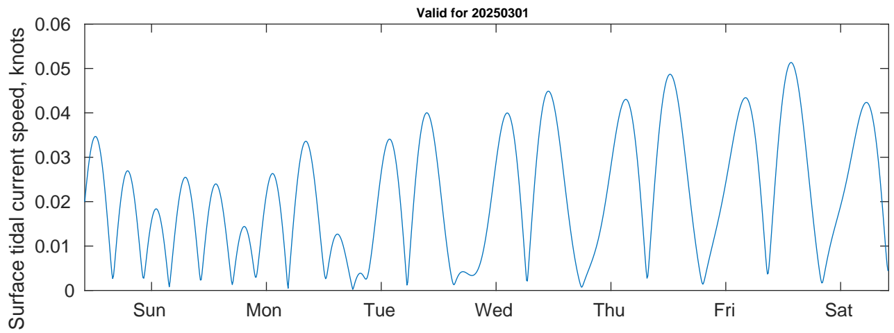
Tidal Currents and Heights for CTI Enbridge Kaskida & Tiber PPL Geotechnical at 20250301
