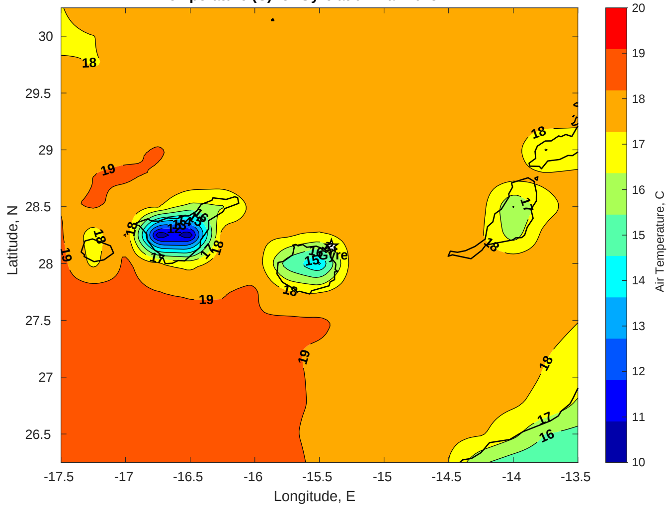
Air Temperature (C) for Gyre at 01-Mar-2025
