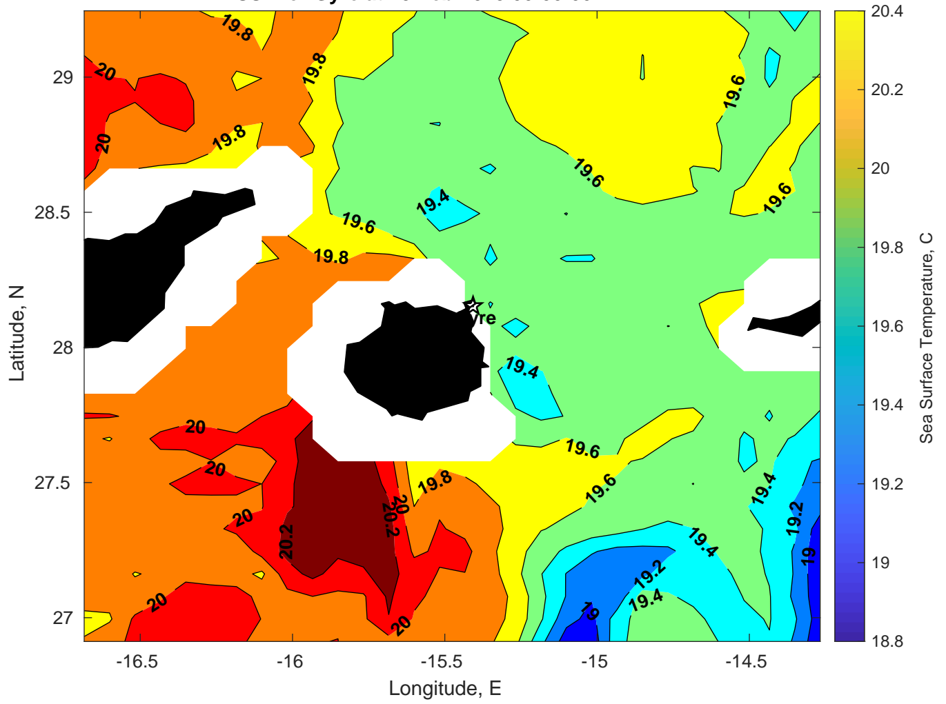
SST for Gyre at 28-Feb-2025 00:00:00
