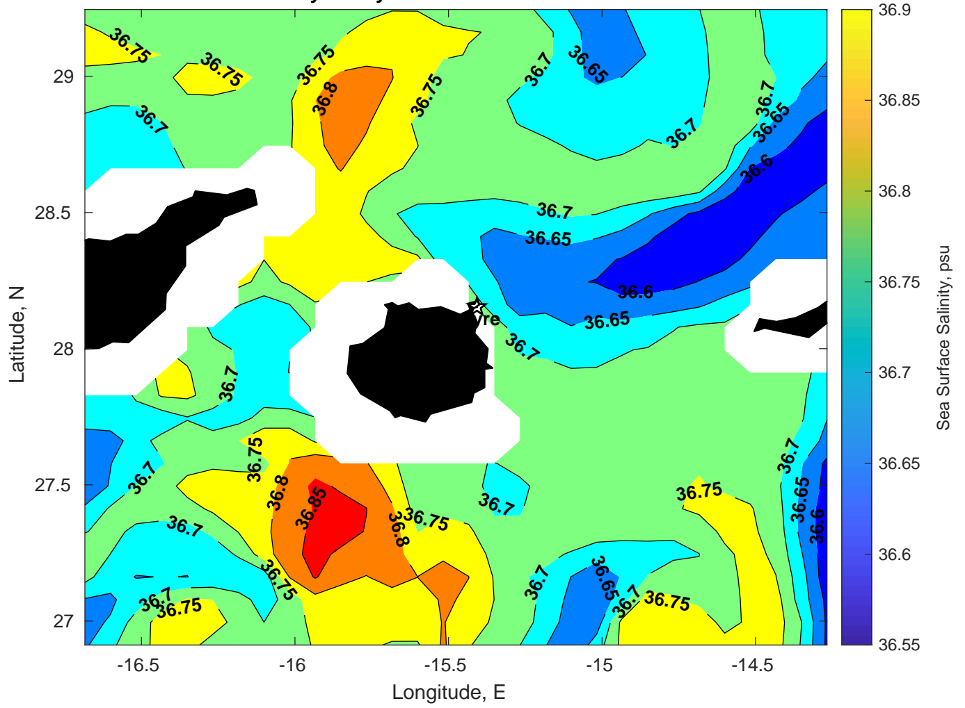
Surface Salinity for Gyre at 28-Feb-2025 00:00:00
