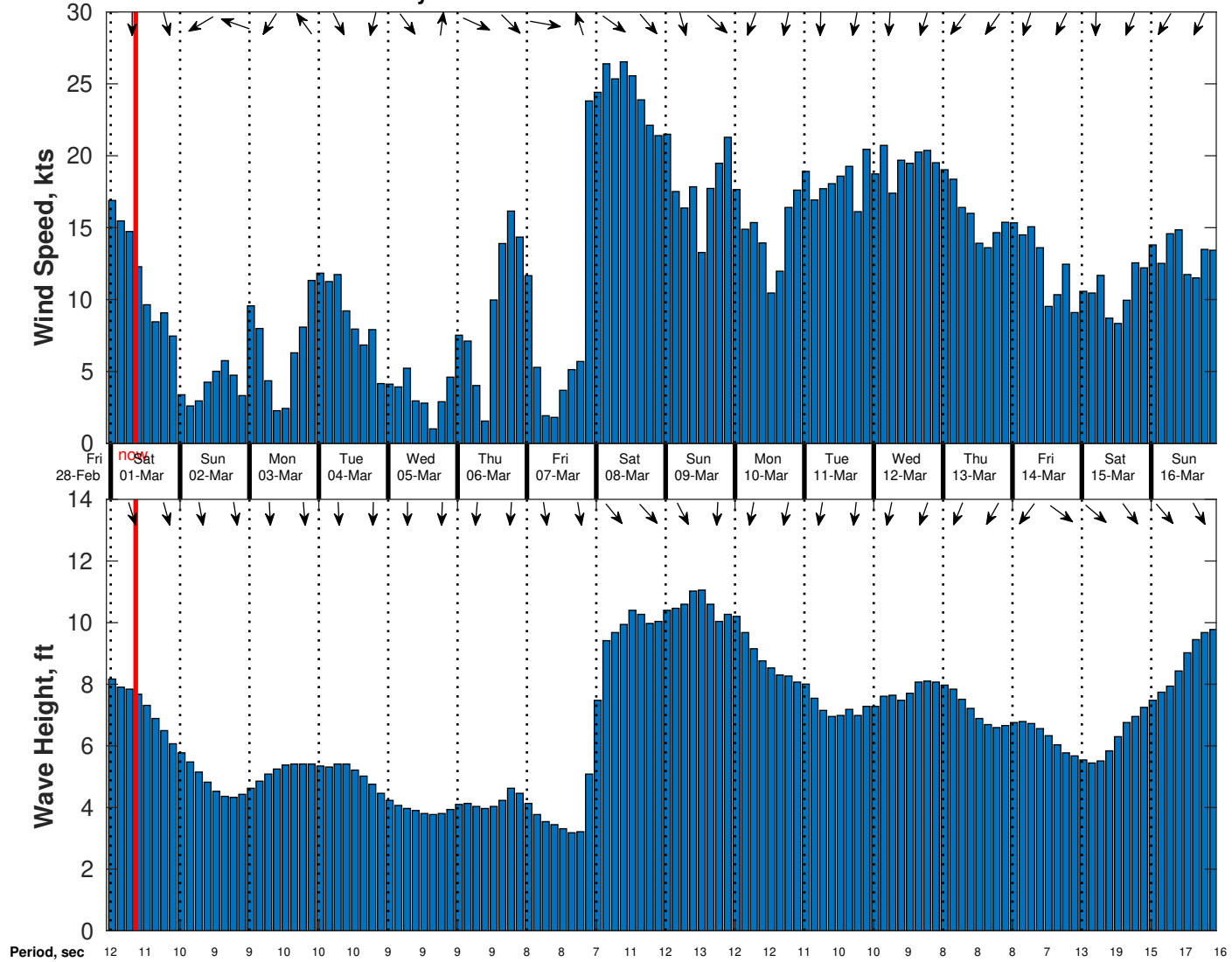
Wind & Wave Forecast for Gyre from 28-Feb-2025 23:00:00 to 16-Mar-2025 23:00:00
