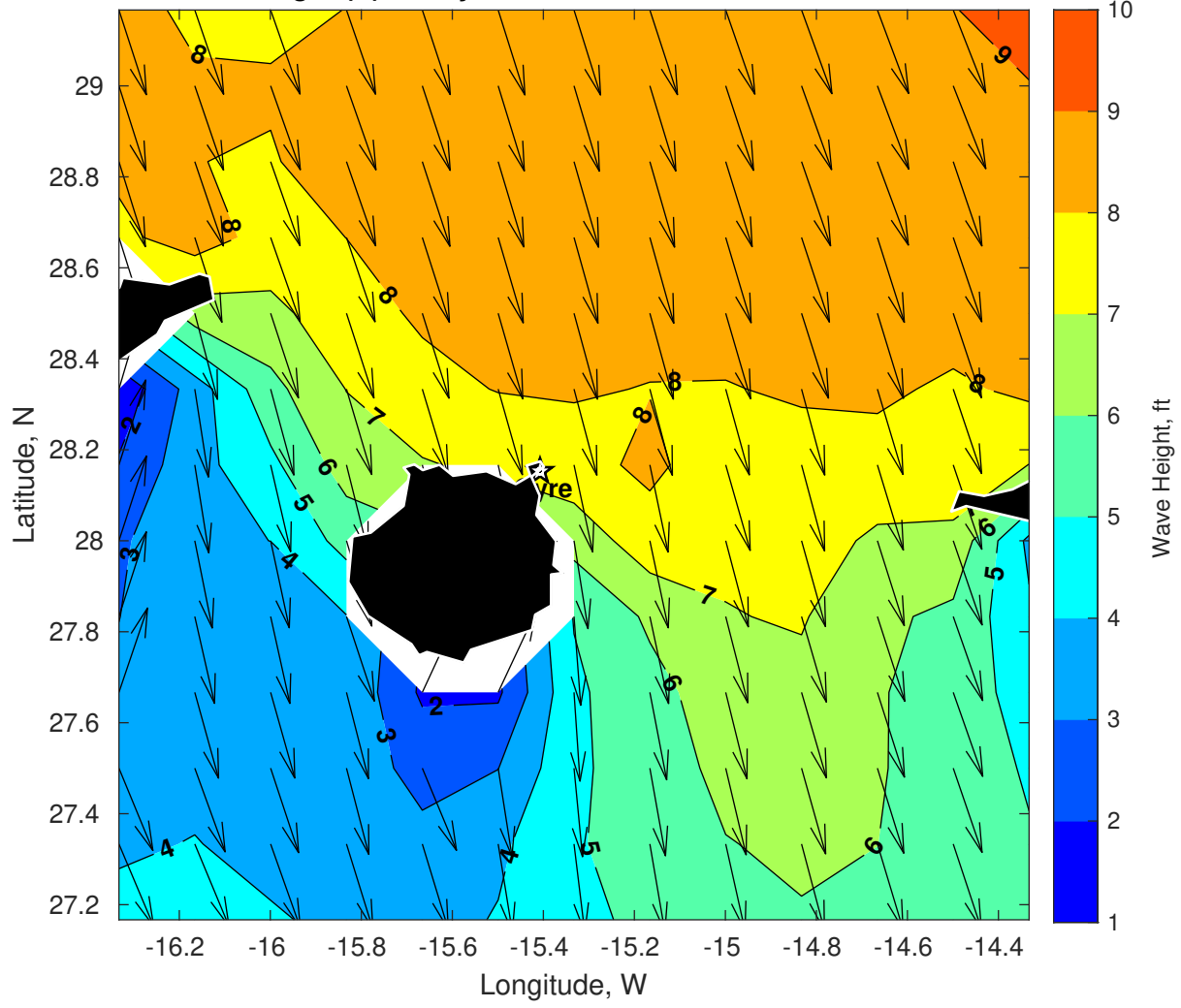
Wave Height (ft) for Gyre at 01-Mar-2025 09:00:00
