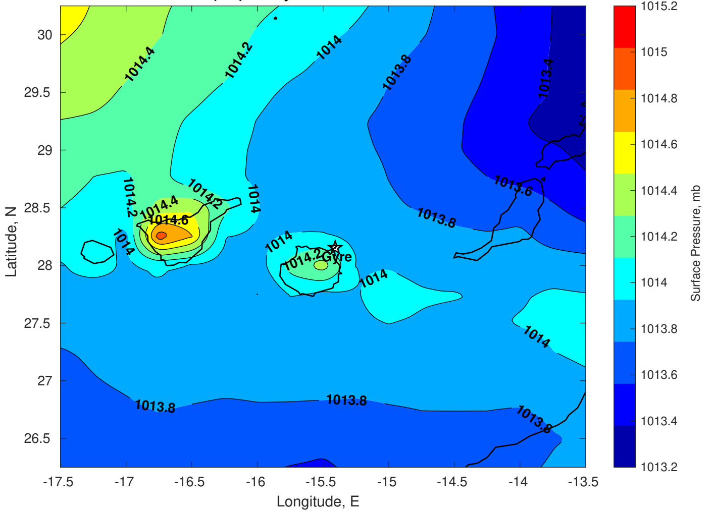
Surface Pressure (mb) for Gyre at 02-Mar-2025 00:00:00
