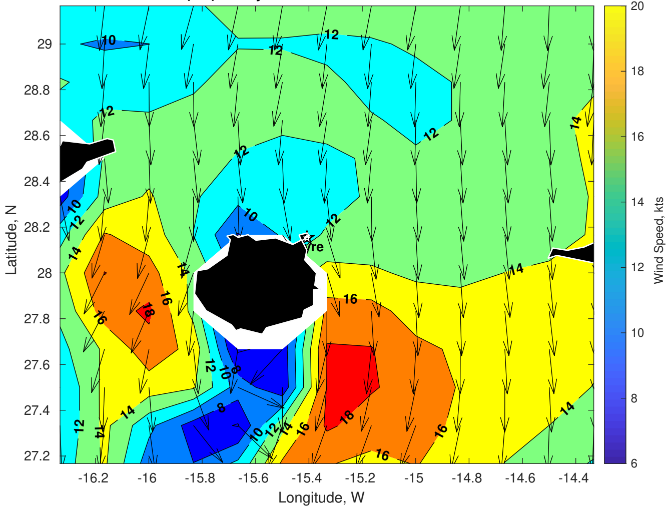
Winds (kts) for Gyre at 01-Mar-2025 09:00:00
