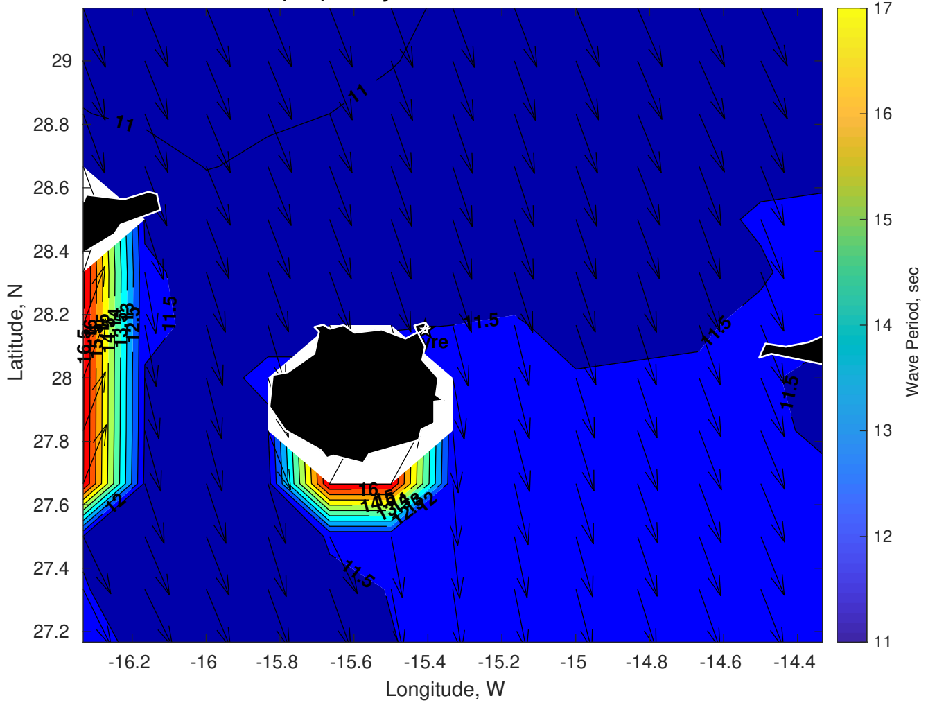
Wave Period (sec) for Gyre at 01-Mar-2025 09:00:00
