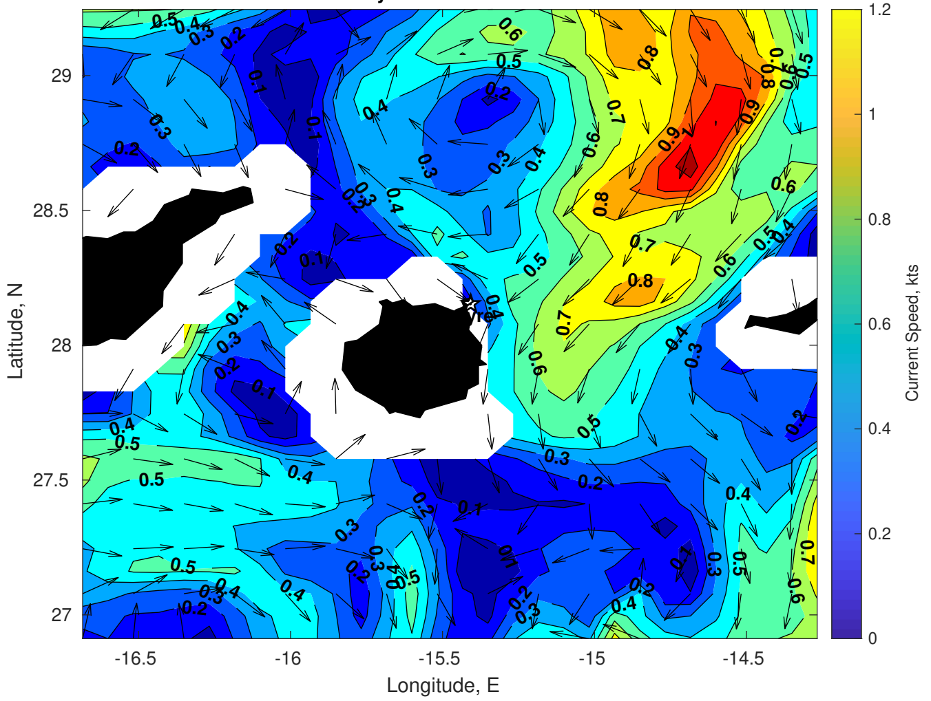
Surface Currents for Gyre at 28-Feb-2025 00:00:00
