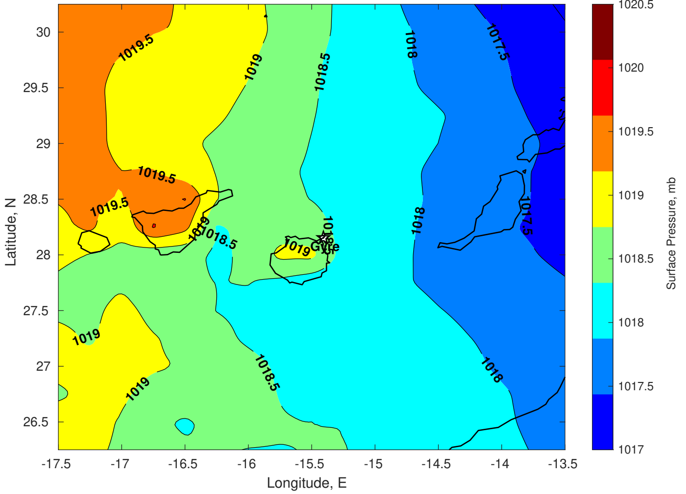
Surface Pressure (mb) for Gyre at 01-Mar-2025 00:00:00
