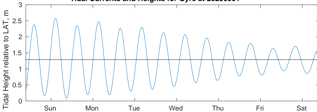
Tidal Currents and Heights for Gyre at 20250301
