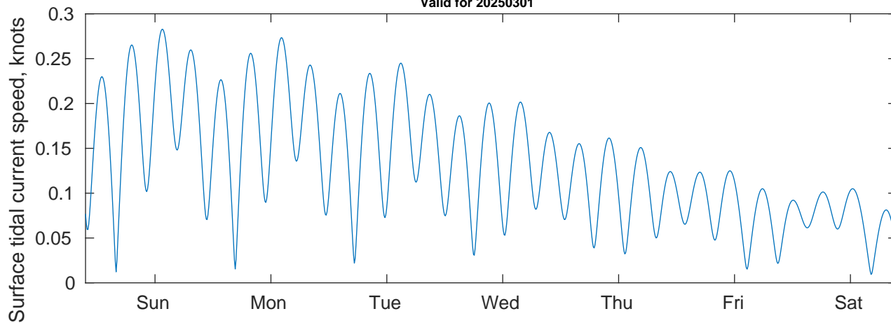
Tidal Currents and Heights for Gyre at 20250301
