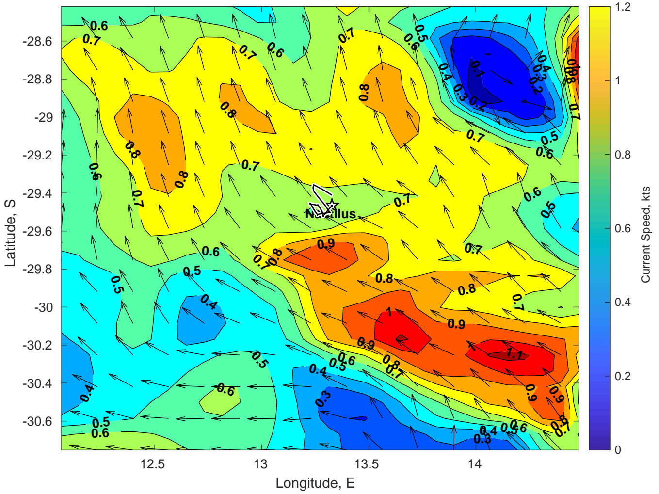
Surface Currents for Nautilus at 28-Feb-2025 00:00:00
