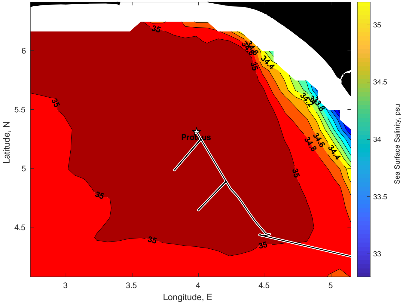
Surface Salinity for Proteus at 28-Feb-2025 00:00:00
