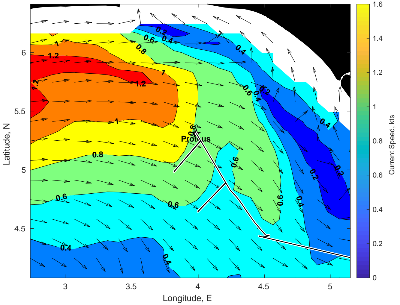
Surface Currents for Proteus at 28-Feb-2025 00:00:00
