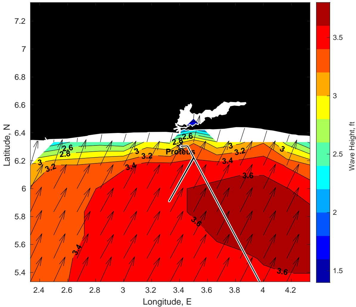
Wave Height (ft) for Proteus at 01-Mar-2025 09:00:00
