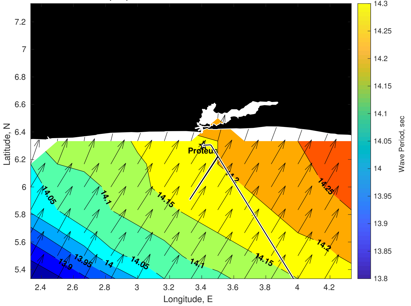
Wave Period (sec) for Proteus at 01-Mar-2025 09:00:00
