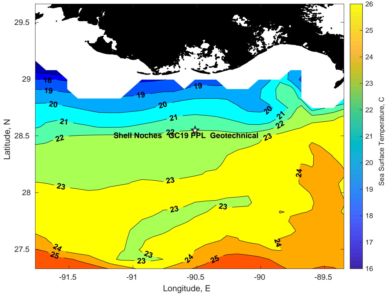
SST for Shell Noches GC19 PPL Geotechnical at 28-Feb-2025 00:00:00
