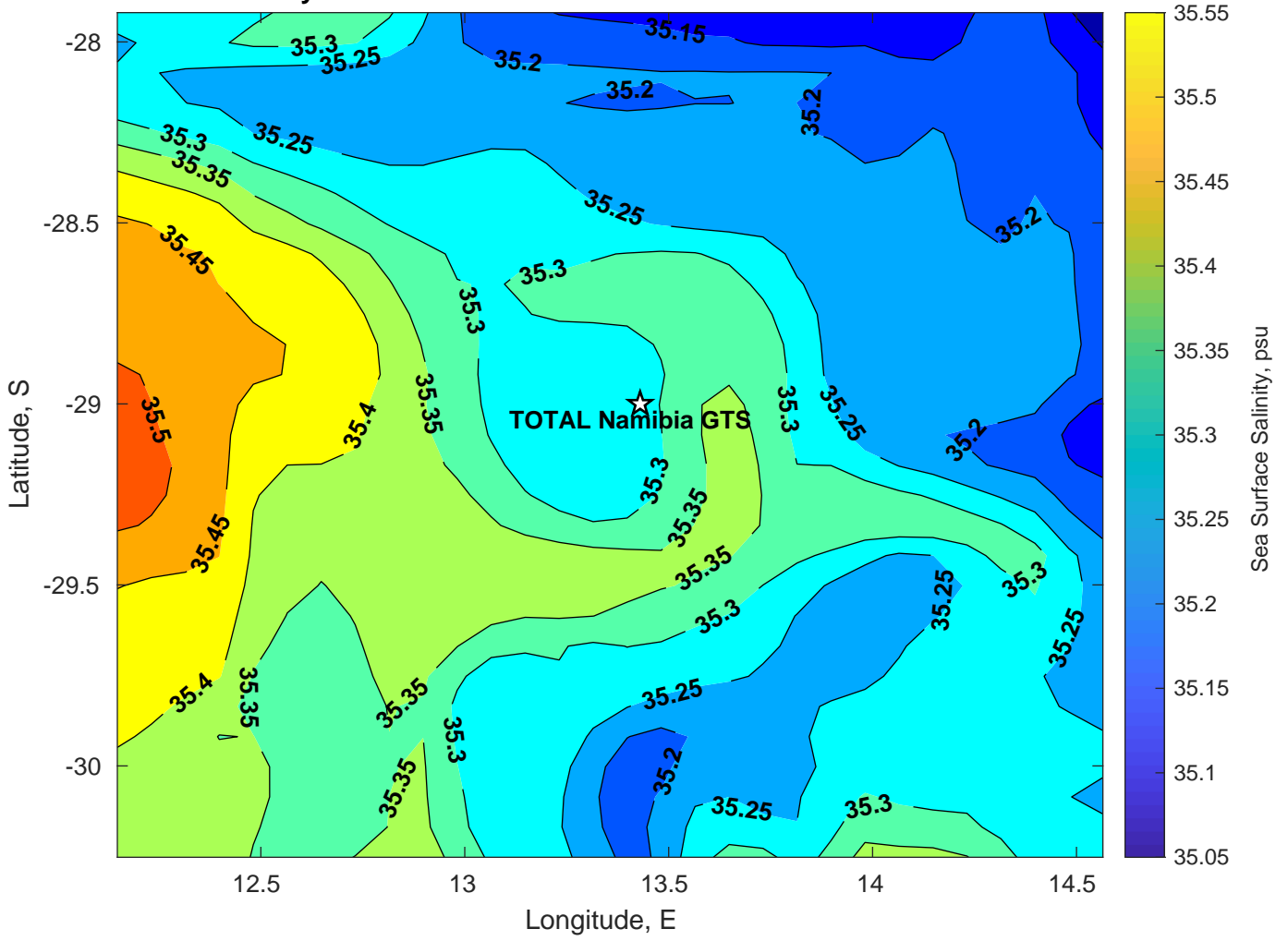
Surface Salinity for TOTAL Namibia GTS at 28-Feb-2025 00:00:00
