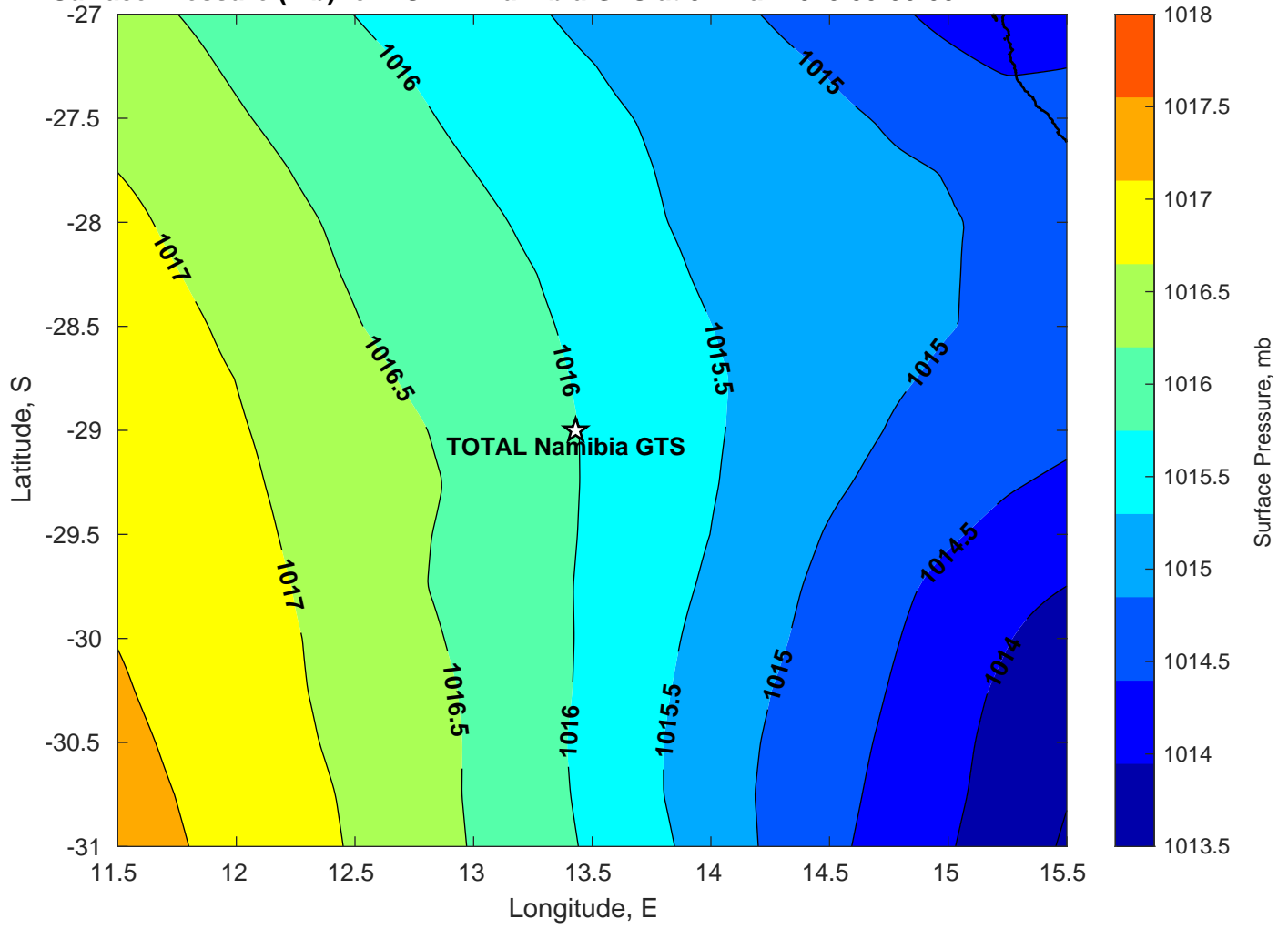
Surface Pressure (mb) for TOTAL Namibia GTS at 01-Mar-2025 00:00:00
