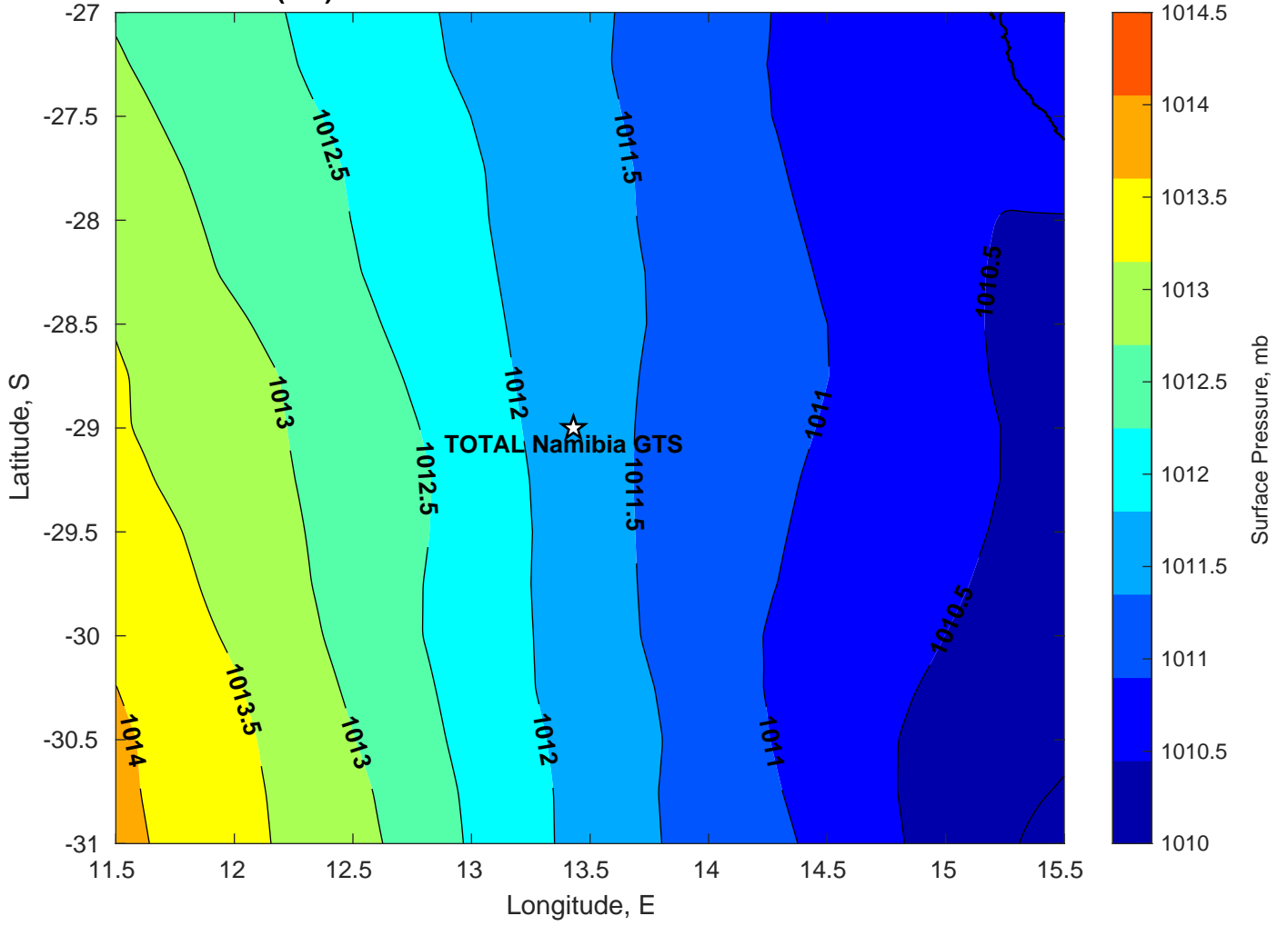
Surface Pressure (mb) for TOTAL Namibia GTS at 03-Mar-2025 00:00:00
