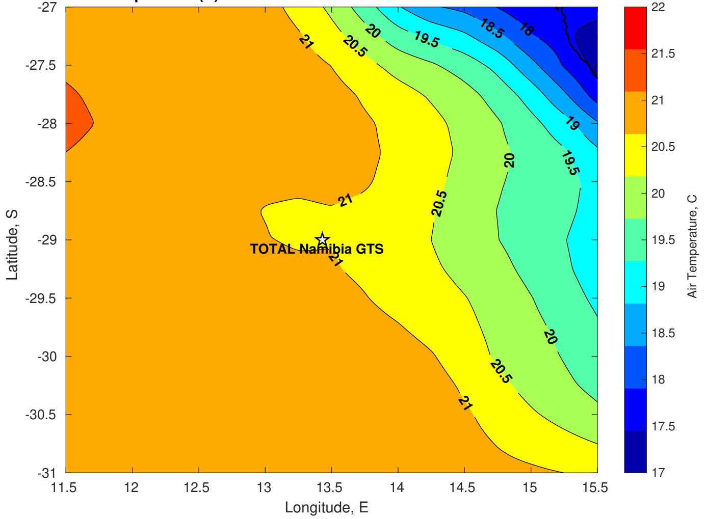
Air Temperature (C) for TOTAL Namibia GTS at 01-Mar-2025
