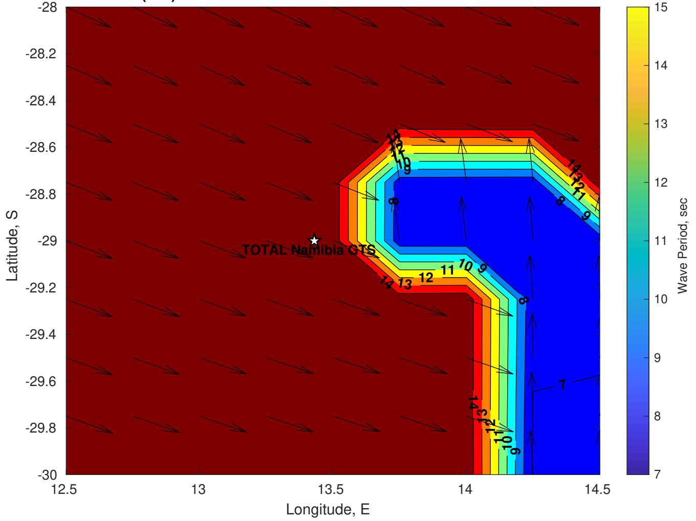
Wave Period (sec) for TOTAL Namibia GTS at 01-Mar-2025 09:00:00
