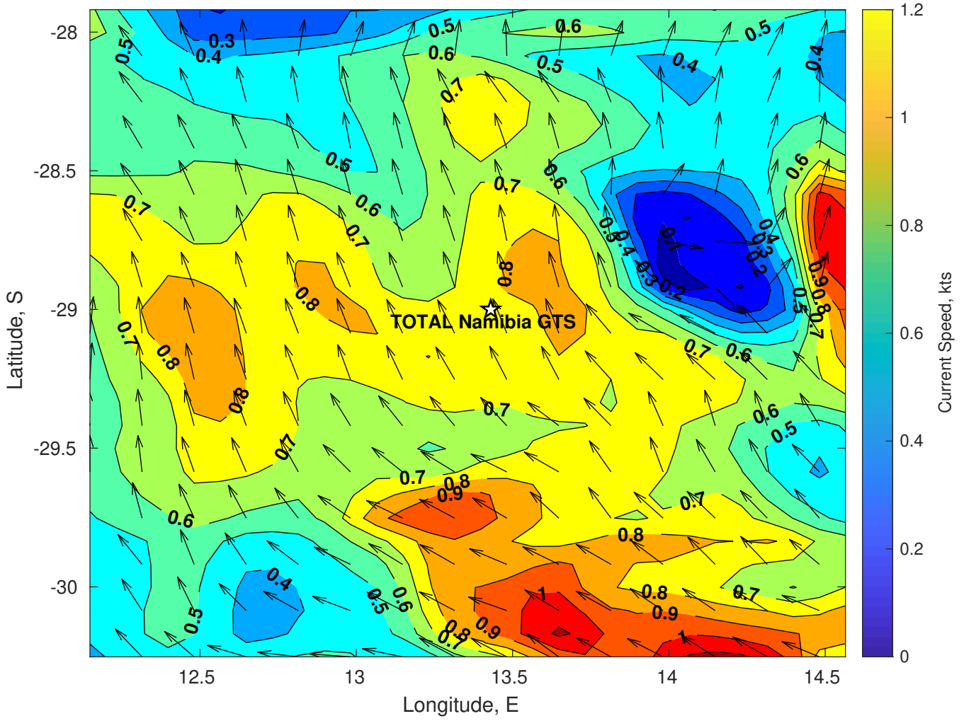
Surface Currents for TOTAL Namibia GTS at 28-Feb-2025 00:00:00
