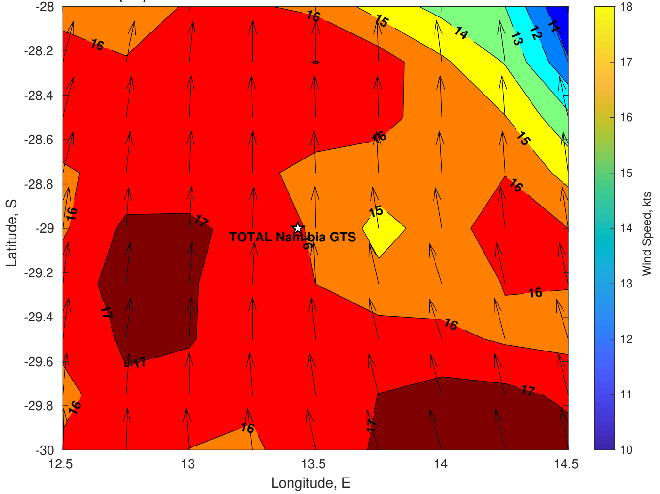
Winds (kts) for TOTAL Namibia GTS at 01-Mar-2025 09:00:00
