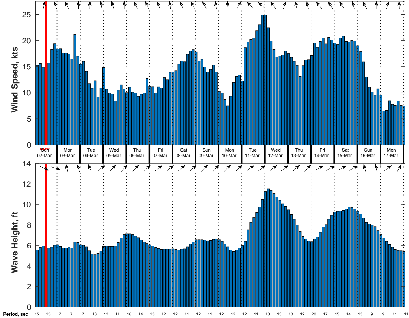
Wind & Wave Forecast for TOTAL Namibia GTS from 01-Mar-2025 02:00:00 to 17-Mar-2025 02:00:00
