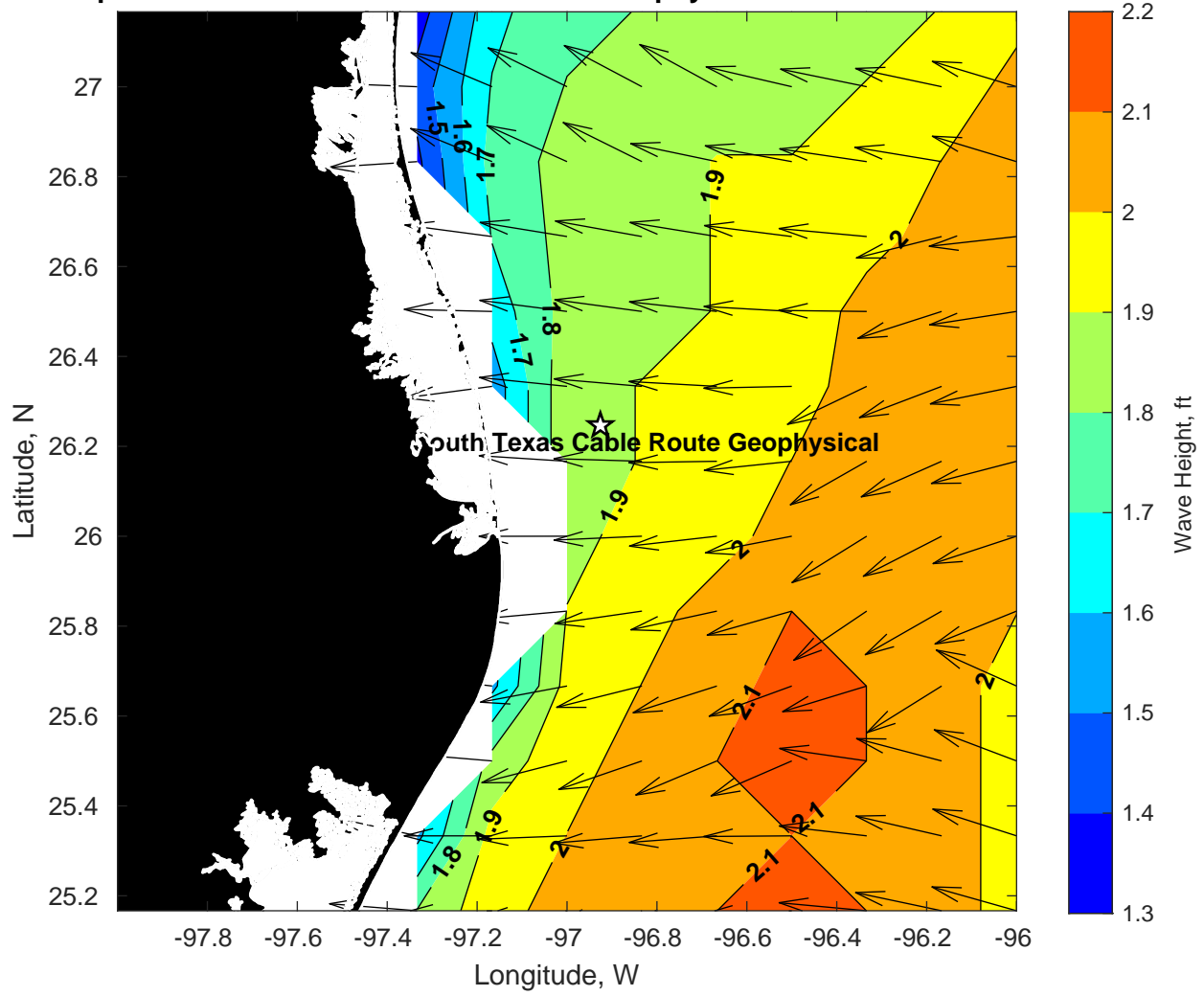
Wave Height (ft) for Tampnet P2378 South Texas Cable Route Geophysical at 01-Mar-2025 09:00:00
