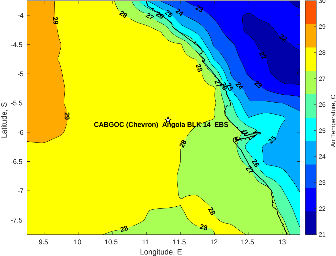
Air Temperature (C) for CABGOC (Chevron) Angola BLK 14 EBS at 02-Mar-2025
