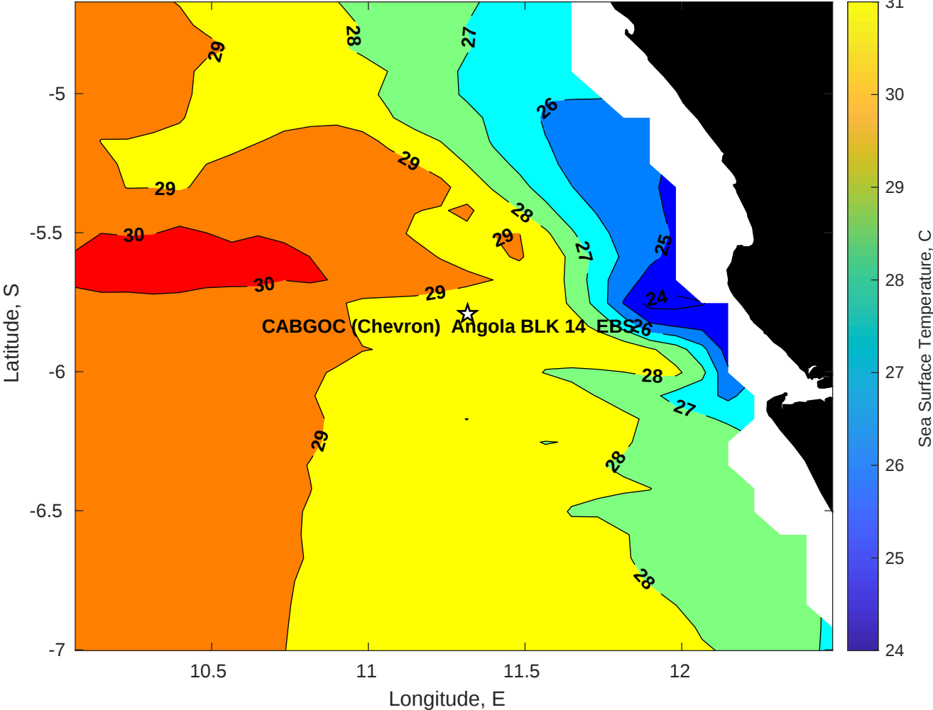
SST for CABGOC (Chevron) Angola BLK 14 EBS at 01-Mar-2025 00:00:00
