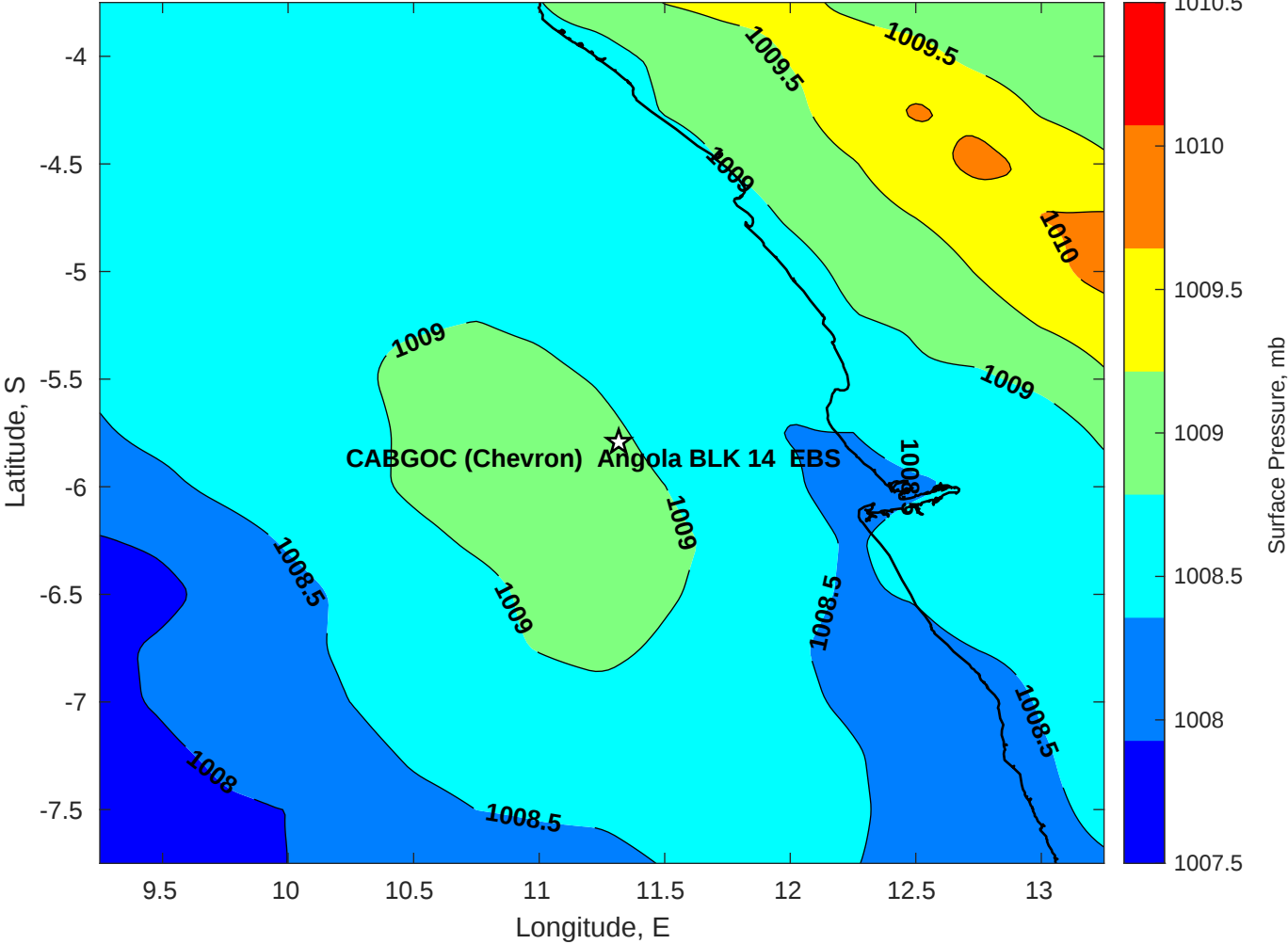
Surface Pressure (mb) for CABGOC (Chevron) Angola BLK 14 EBS at 04-Mar-2025 00:00:00
