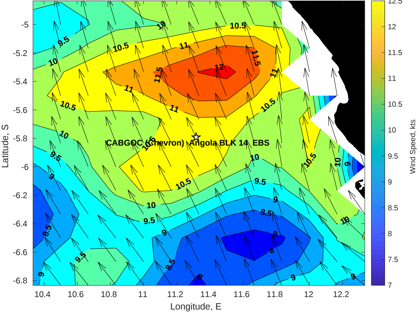
Winds (kts) for CABGOC (Chevron) Angola BLK 14 EBS at 02-Mar-2025 09:00:00
