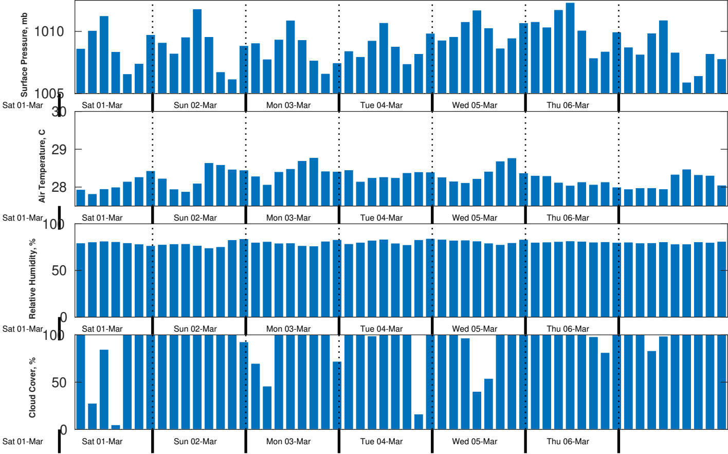
Met Forecast for CABGOC (Chevron) Angola BLK 14 EBS from 02-Mar-2025 00:00:00 to 09-Mar-2025 00:00:00
