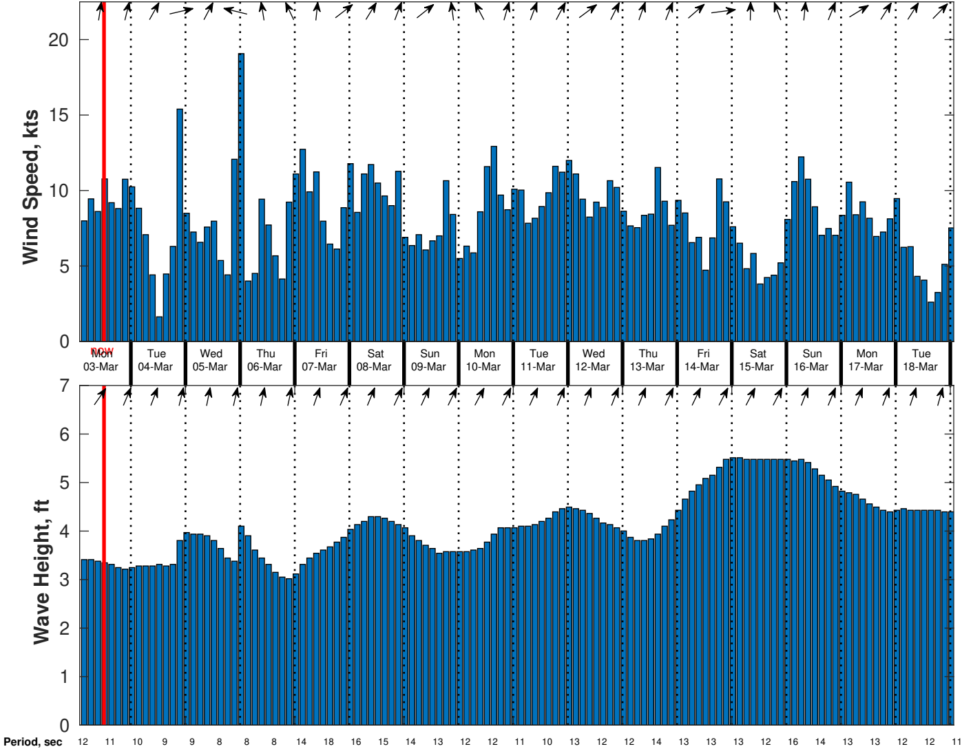
Wind & Wave Forecast for CABGOC (Chevron) Angola BLK 14 EBS from 02-Mar-2025 02:00:00 to 18-Mar-2025 02:00:00
