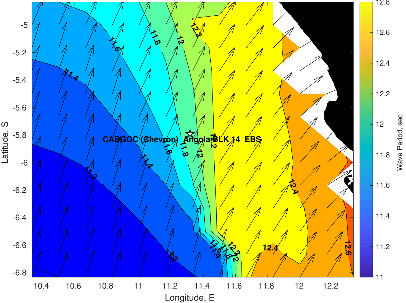
Wave Period (sec) for CABGOC (Chevron) Angola BLK 14 EBS at 02-Mar-2025 09:00:00
