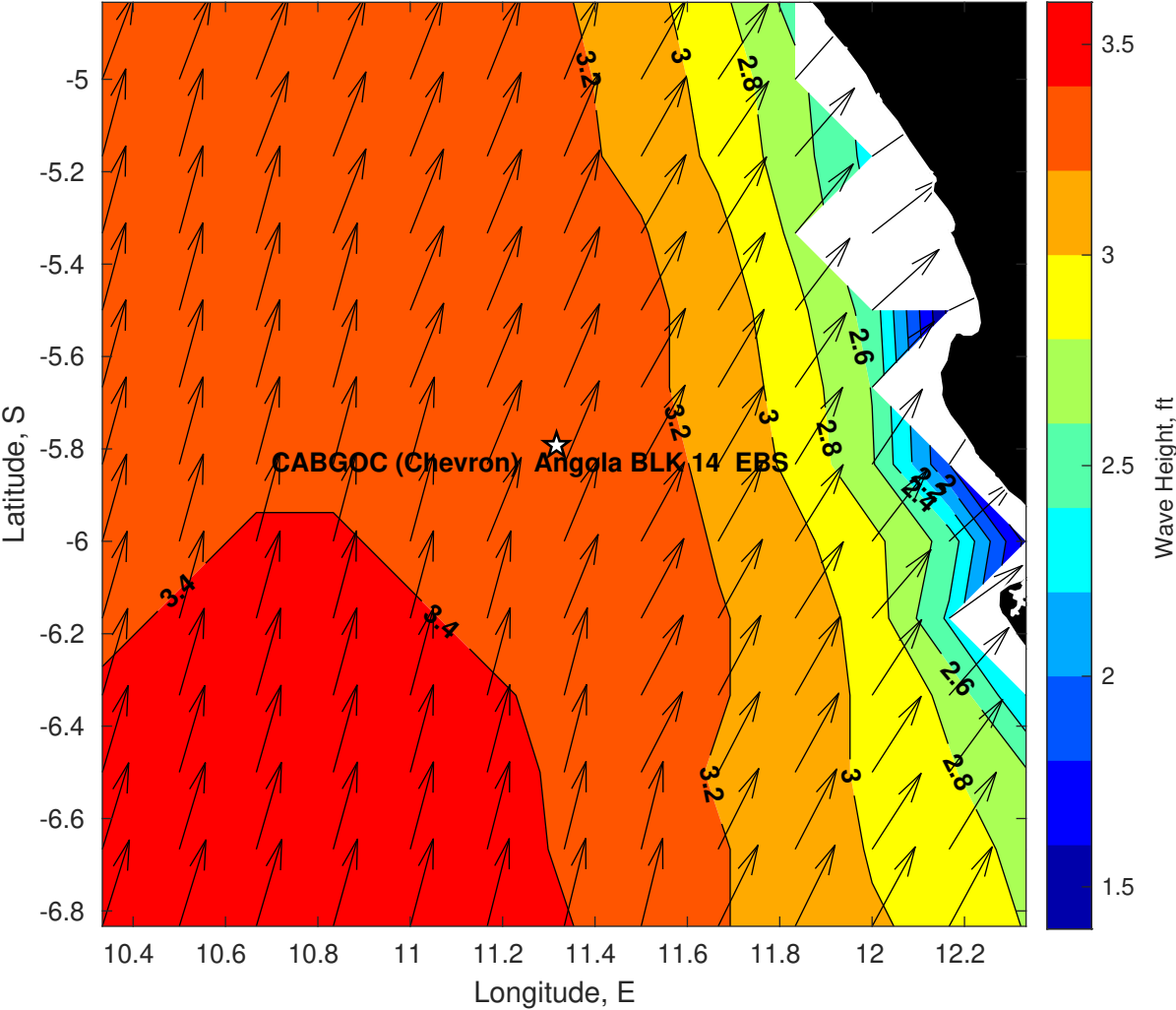
Wave Height (ft) for CABGOC (Chevron) Angola BLK 14 EBS at 02-Mar-2025 09:00:00
