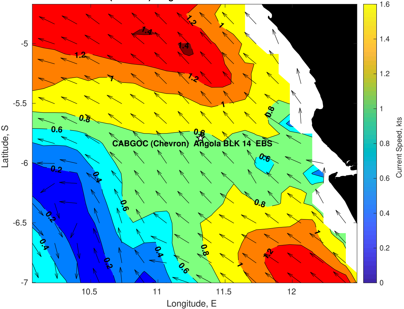
Surface Currents for CABGOC (Chevron) Angola BLK 14 EBS at 01-Mar-2025 00:00:00
