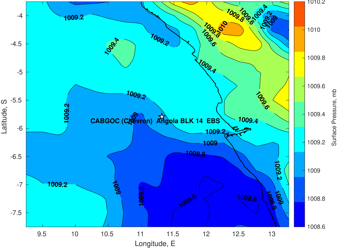
Surface Pressure (mb) for CABGOC (Chevron) Angola BLK 14 EBS at 03-Mar-2025 00:00:00
