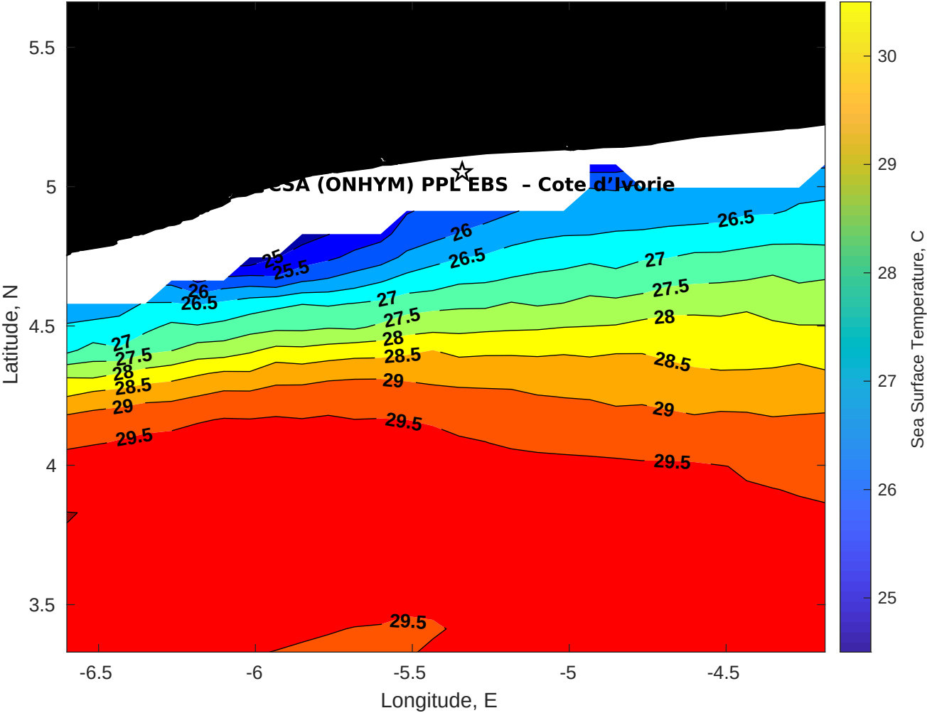
SST for CSA (ONHYM) PPL EBS - Cote d'Ivoire at 01-Mar-2025 00:00:00
