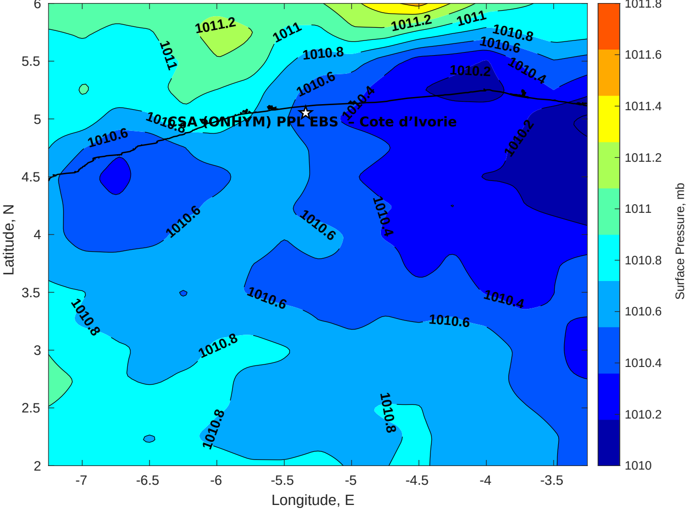
Surface Pressure (mb) for CSA (ONHYM) PPL EBS - Cote d'Ivoire at 02-Mar-2025 00:00:00
