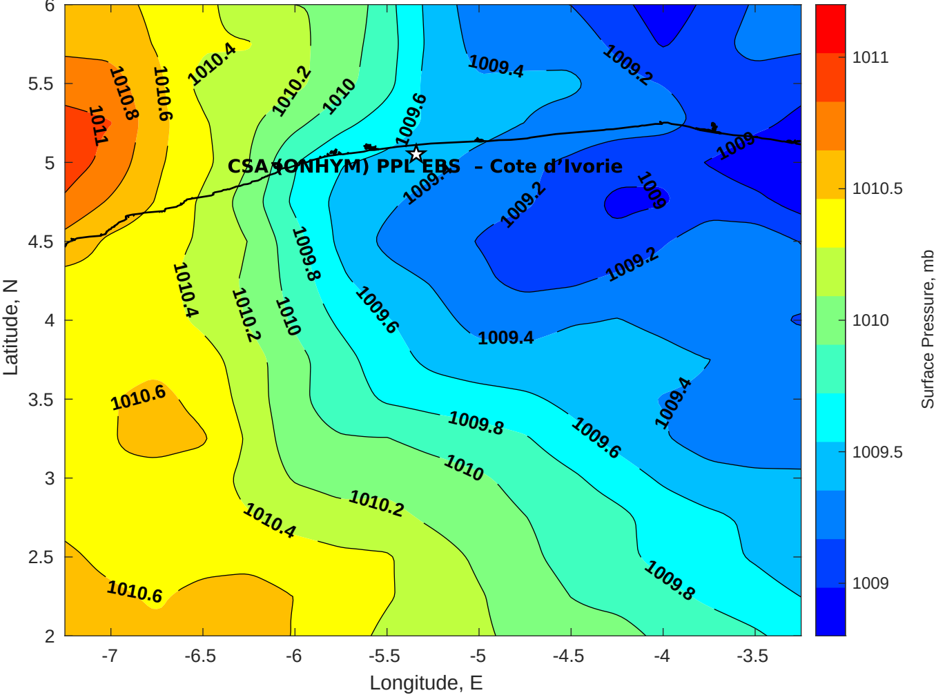
Surface Pressure (mb) for CSA (ONHYM) PPL EBS - Cote d'Ivoire at 04-Mar-2025 00:00:00
