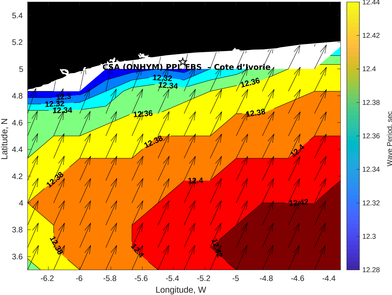
Wave Period (sec) for CSA (ONHYM) PPL EBS - Cote d'Ivoire at 02-Mar-2025 09:00:00
