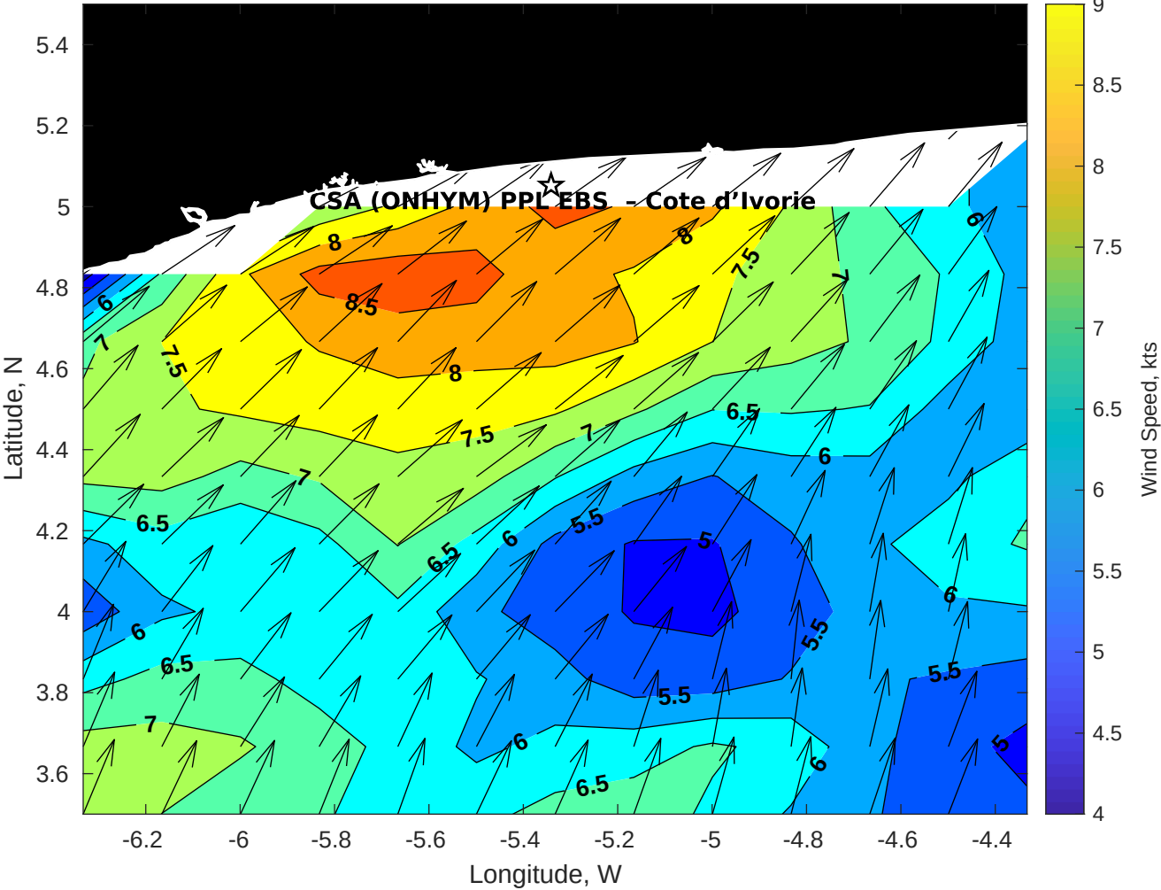
Winds (kts) for CSA (ONHYM) PPL EBS - Cote d'Ivoire at 02-Mar-2025 09:00:00
