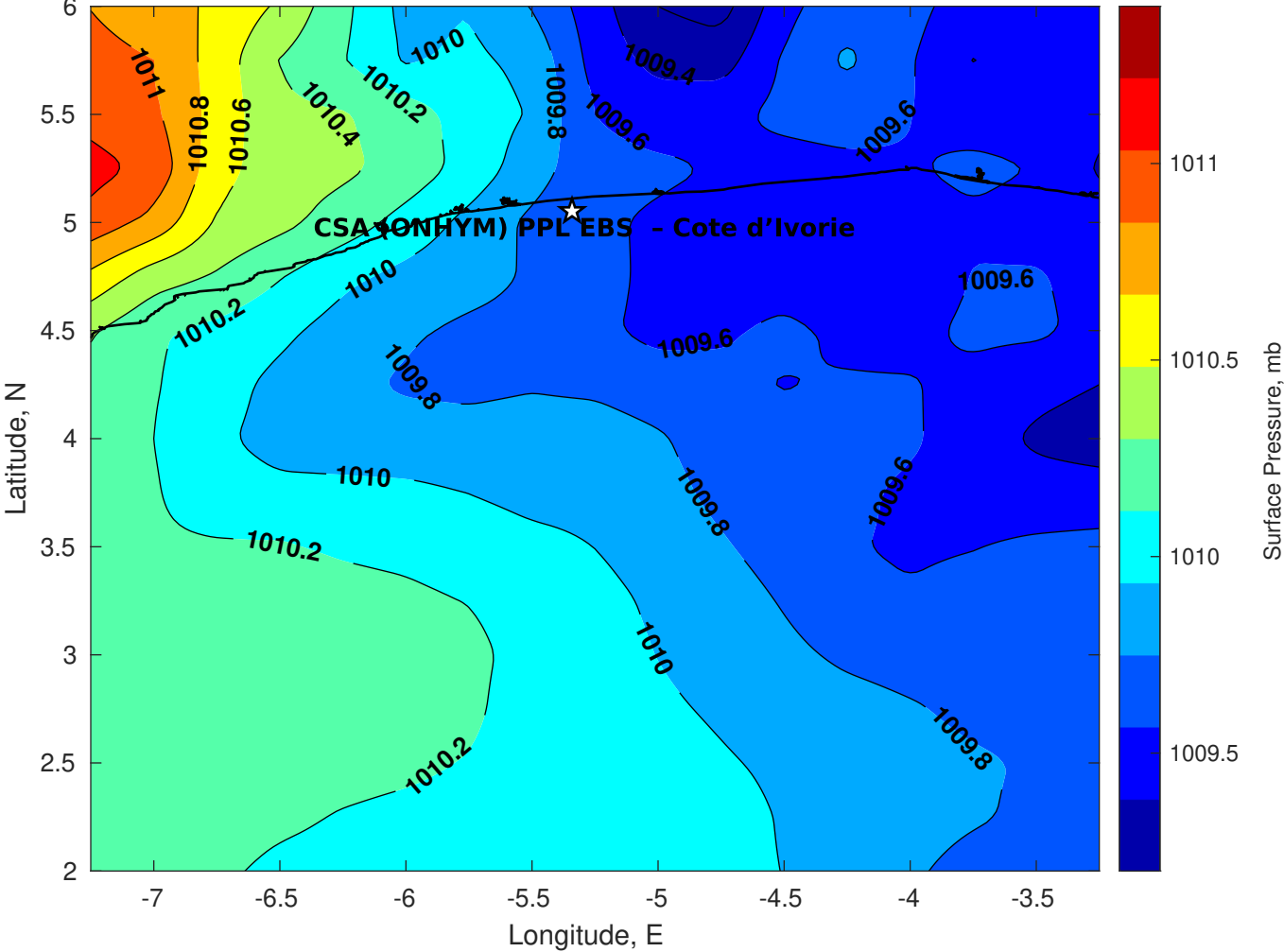
Surface Pressure (mb) for CSA (ONHYM) PPL EBS - Cote d'Ivoire at 03-Mar-2025 00:00:00
