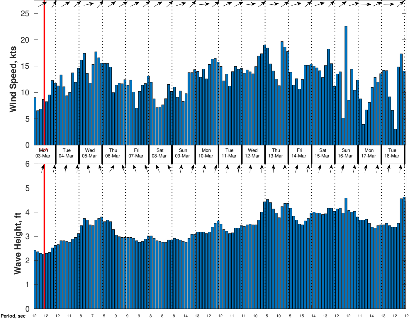
Wind & Wave Forecast for CSA (ONHYM) PPL EBS - Cote d'Ivoire from 02-Mar-2025 01:00:00 to 18-Mar-2025 01:00:00
