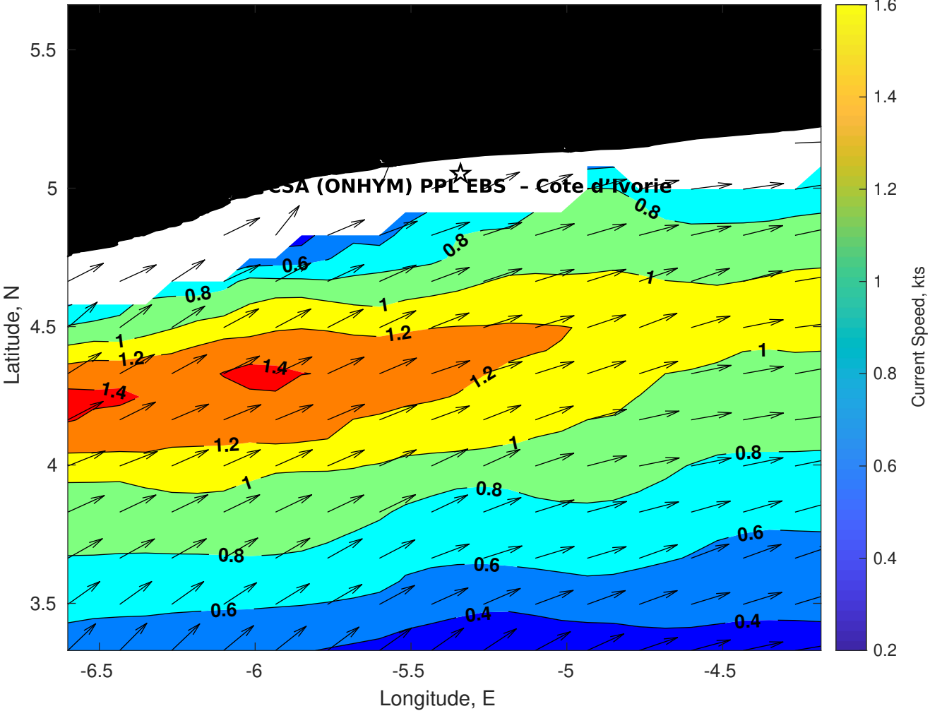
Surface Currents for CSA (ONHYM) PPL EBS - Cote d'Ivoire at 01-Mar-2025 00:00:00
