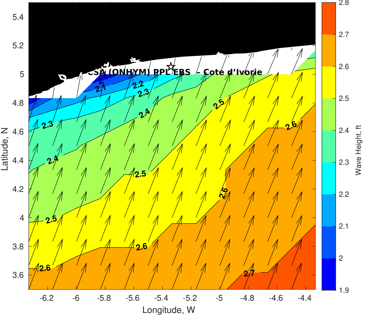
Wave Height (ft) for CSA (ONHYM) PPL EBS - Cote d'Ivoire at 02-Mar-2025 09:00:00
