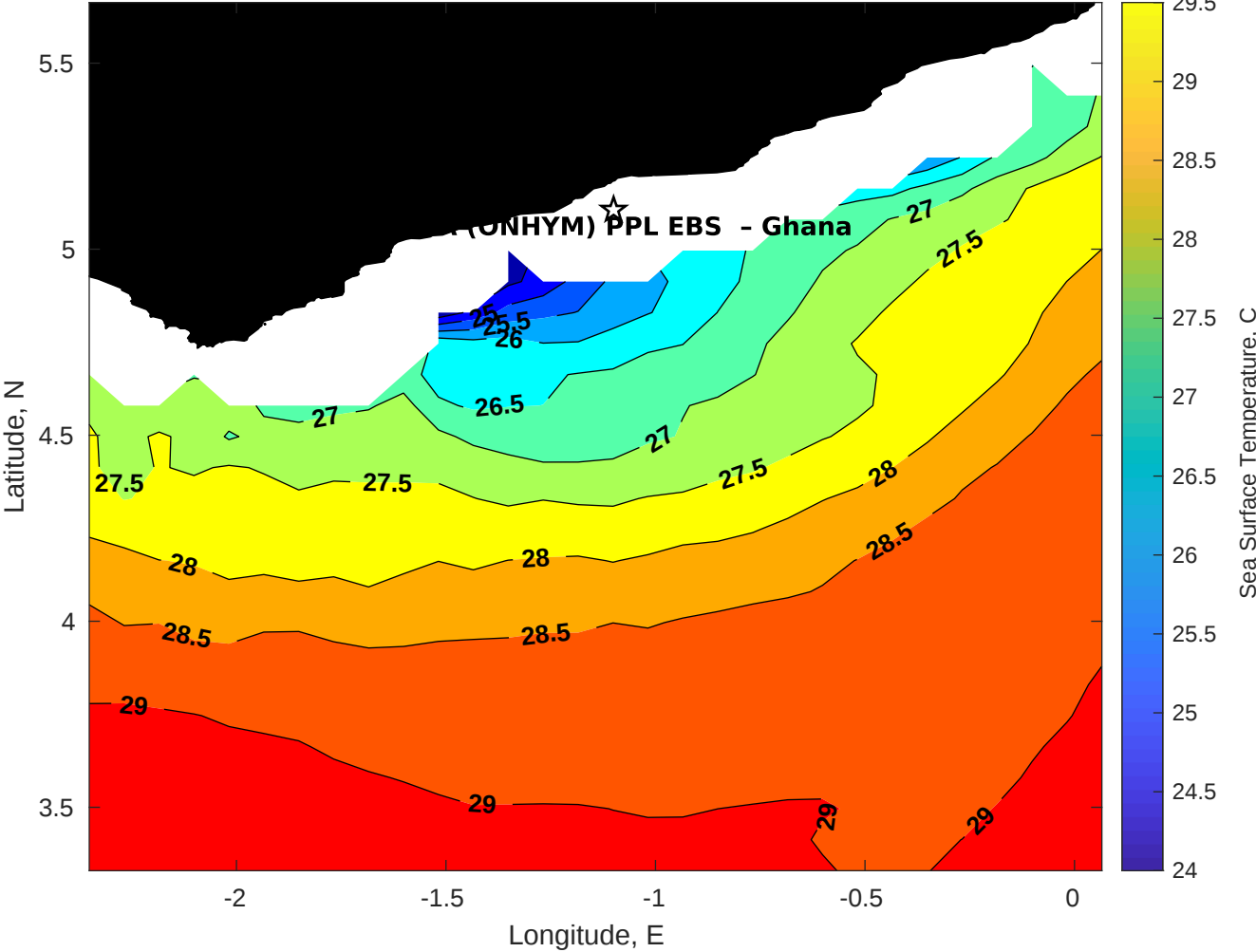
SST for CSA (ONHYM) PPL EBS - Ghana at 01-Mar-2025 00:00:00
