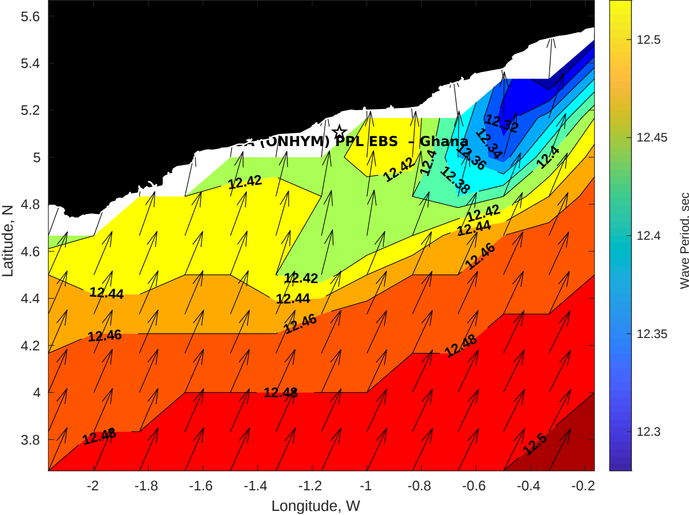
Wave Period (sec) for CSA (ONHYM) PPL EBS - Ghana at 02-Mar-2025 09:00:00
