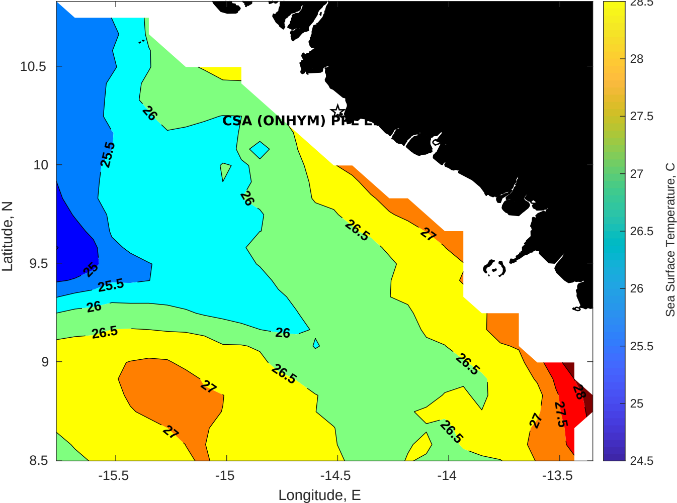
SST for CSA (ONHYM) PPL EBS - Guinea at 01-Mar-2025 00:00:00
