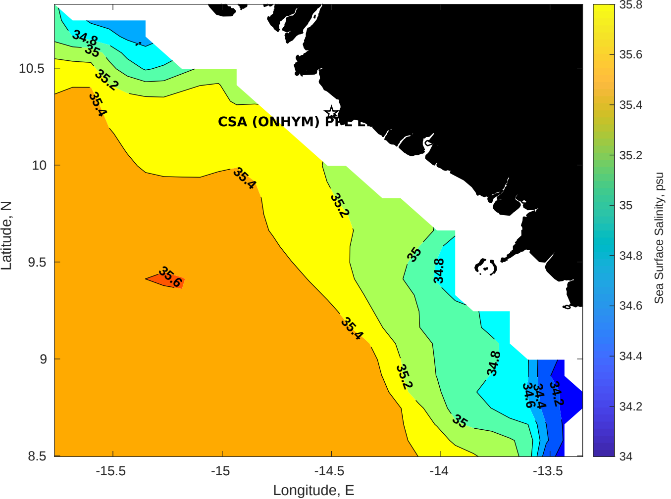
Surface Salinity for CSA (ONHYM) PPL EBS - Guinea at 01-Mar-2025 00:00:00
