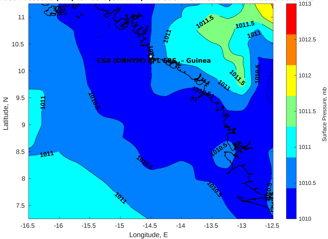
Surface Pressure (mb) for CSA (ONHYM) PPL EBS - Guinea at 02-Mar-2025 00:00:00
