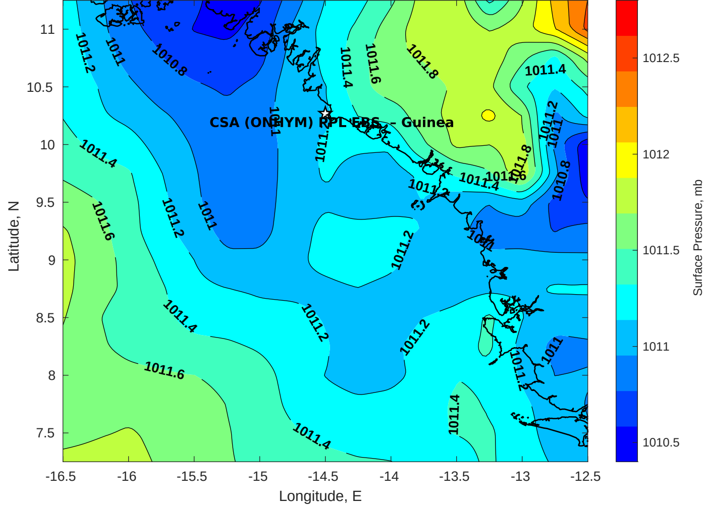
Surface Pressure (mb) for CSA (ONHYM) PPL EBS - Guinea at 03-Mar-2025 00:00:00
