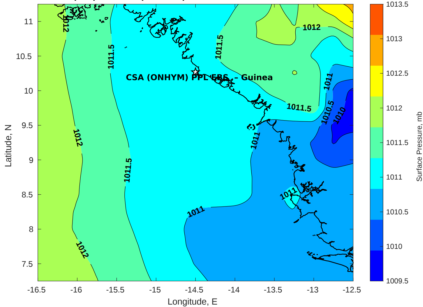
Surface Pressure (mb) for CSA (ONHYM) PPL EBS - Guinea at 04-Mar-2025 00:00:00
