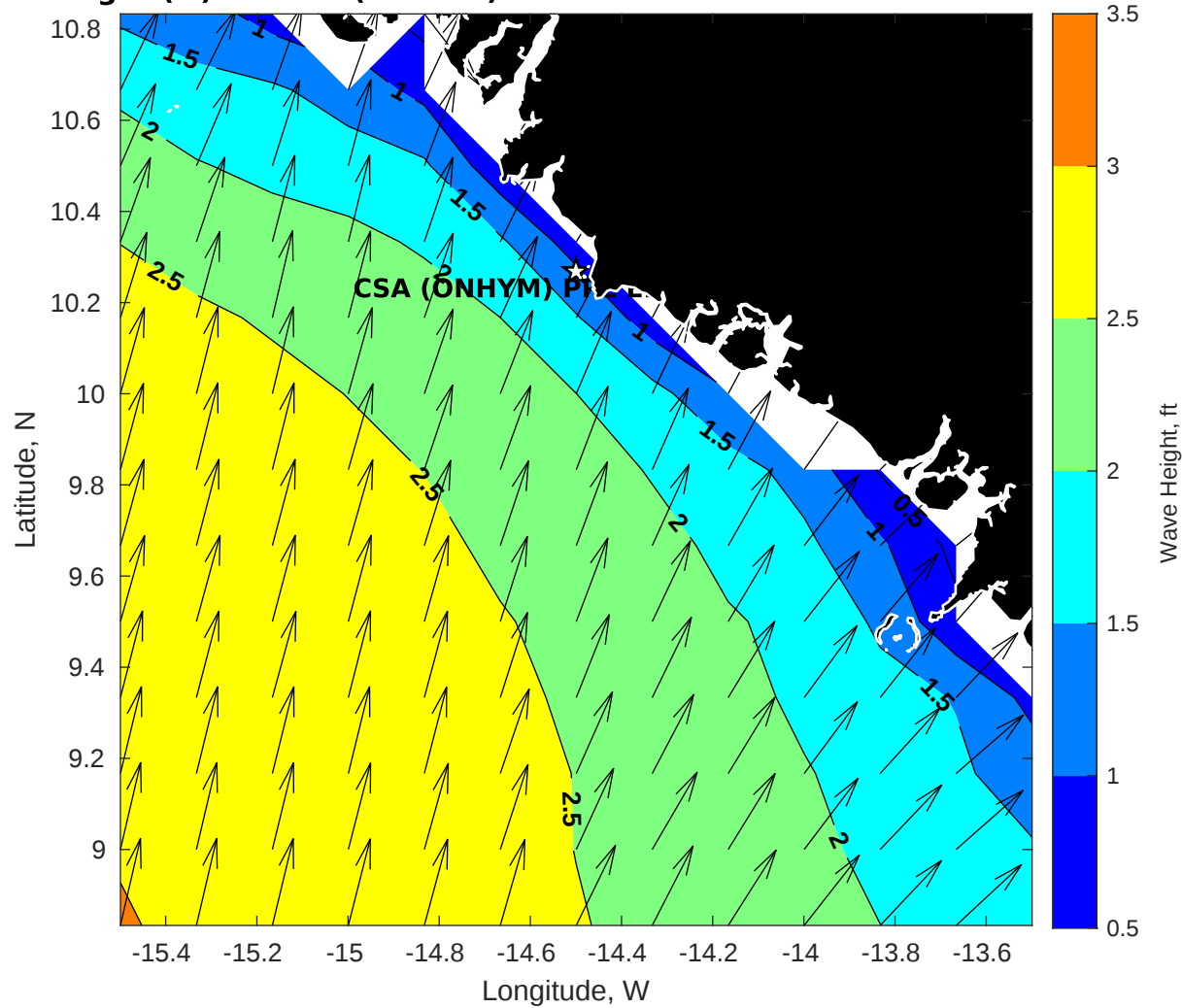
Wave Height (ft) for CSA (ONHYM) PPL EBS - Guinea at 02-Mar-2025 09:00:00
