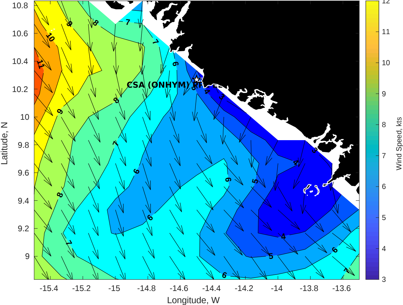
Winds (kts) for CSA (ONHYM) PPL EBS - Guinea at 02-Mar-2025 09:00:00
