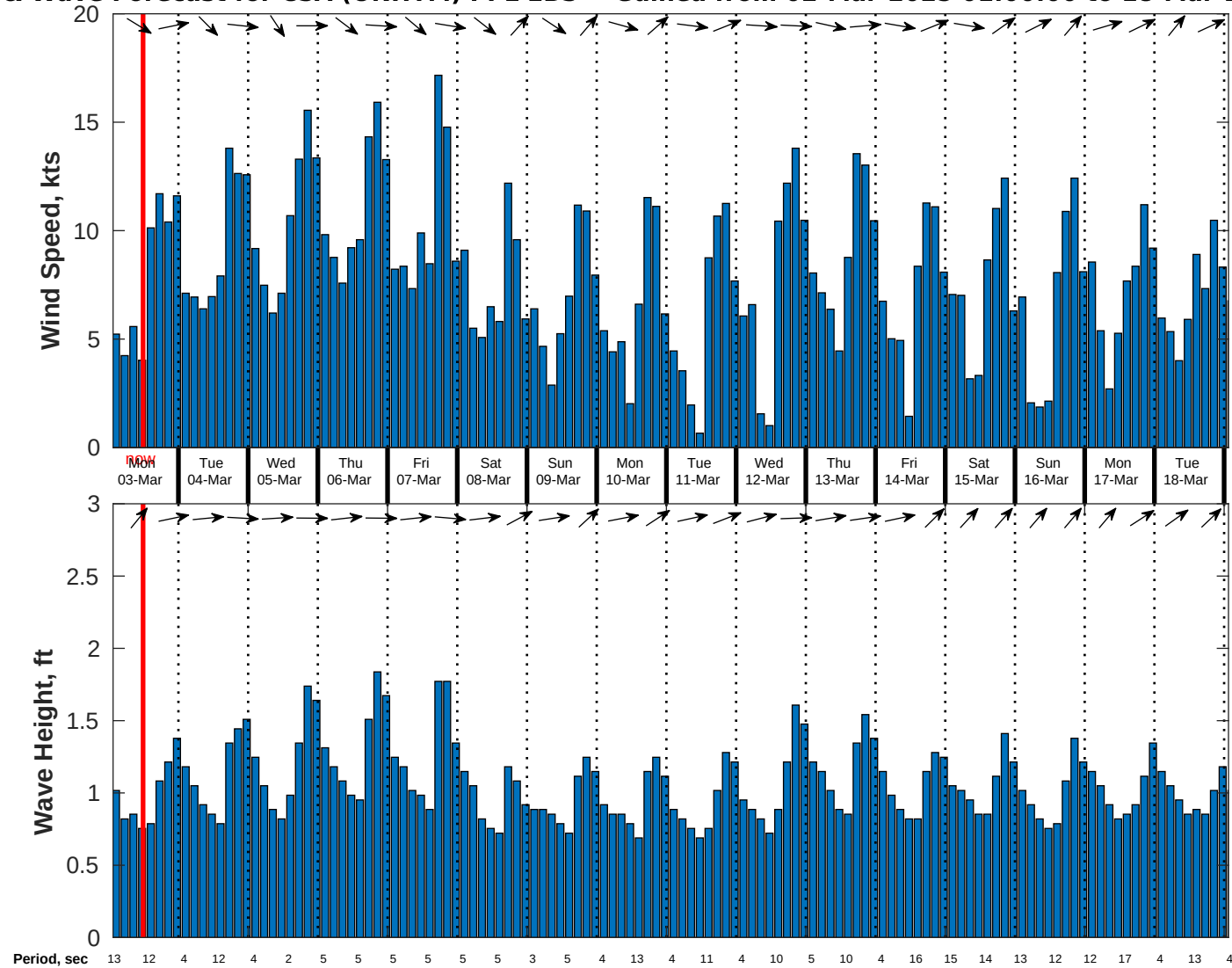
Wind & Wave Forecast for CSA (ONHYM) PPL EBS - Guinea from 02-Mar-2025 01:00:00 to 18-Mar-2025 01:00:00
