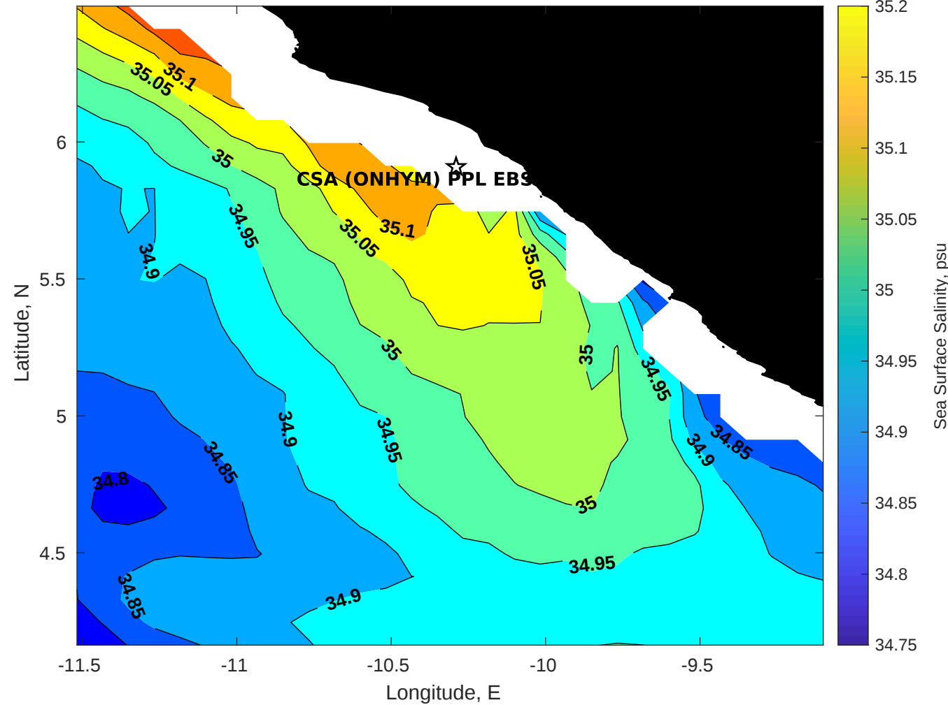
Surface Salinity for CSA (ONHYM) PPL EBS - Liberia at 01-Mar-2025 00:00:00
