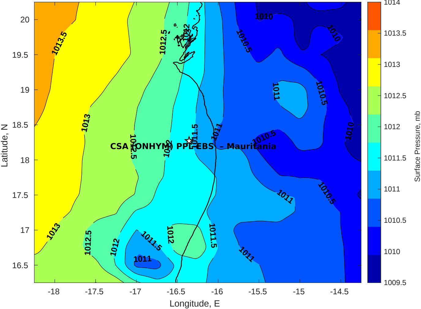
Surface Pressure (mb) for CSA (ONHYM) PPL EBS - Mauritania at 02-Mar-2025 00:00:00
