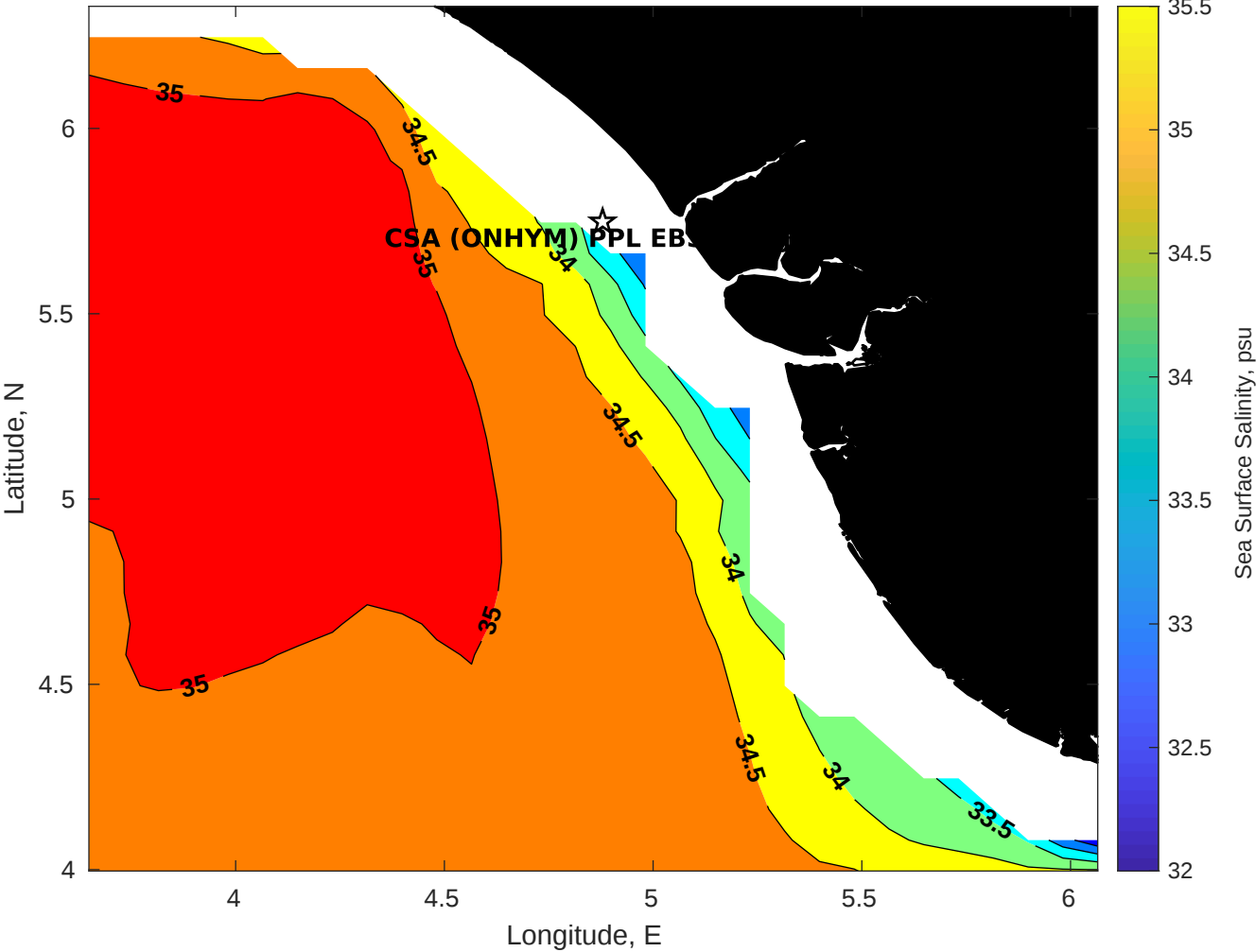
Surface Salinity for CSA (ONHYM) PPL EBS - Nigeria at 01-Mar-2025 00:00:00
