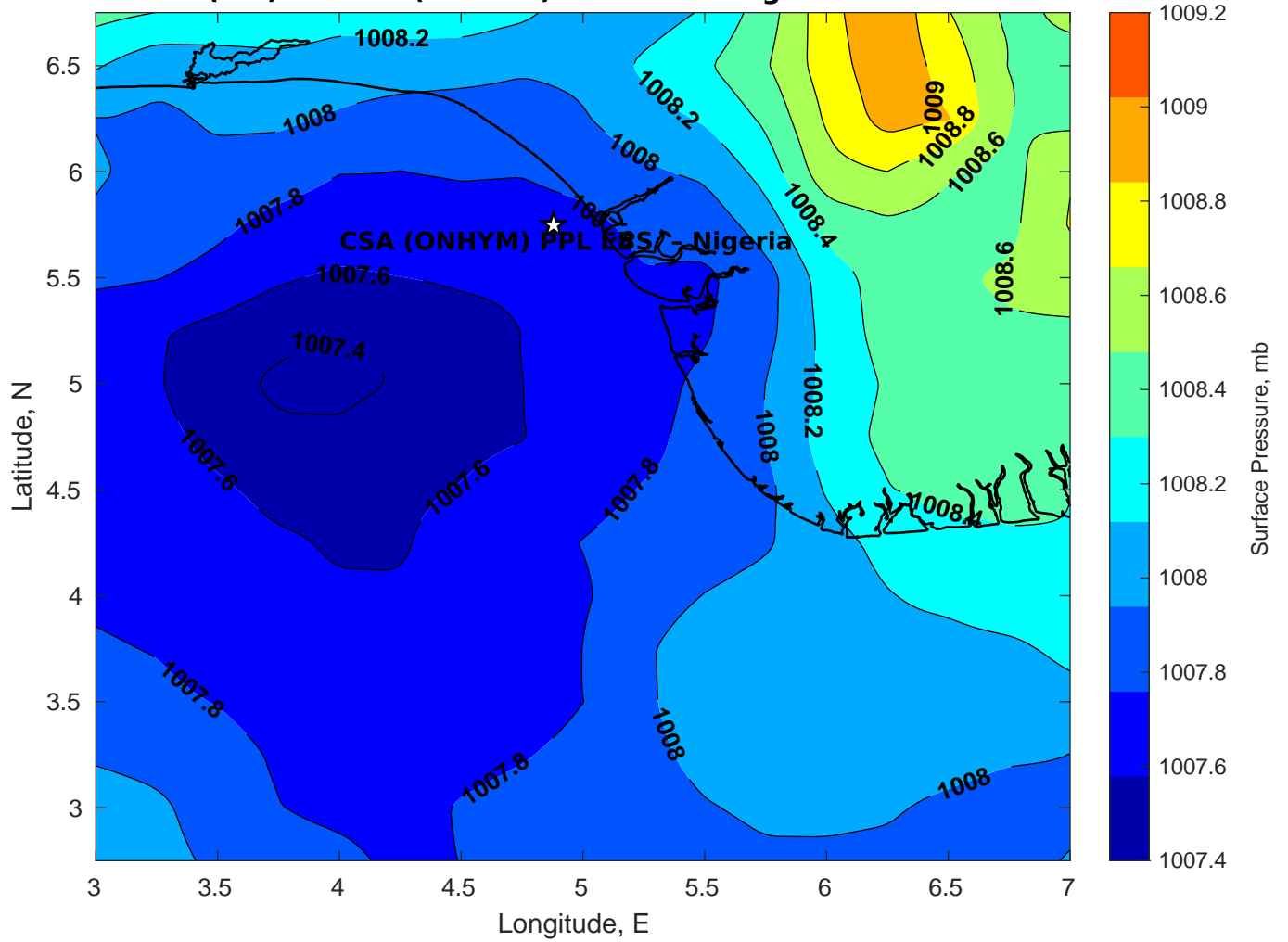
Surface Pressure (mb) for CSA (ONHYM) PPL EBS - Nigeria at 03-Mar-2025 06:00:00
