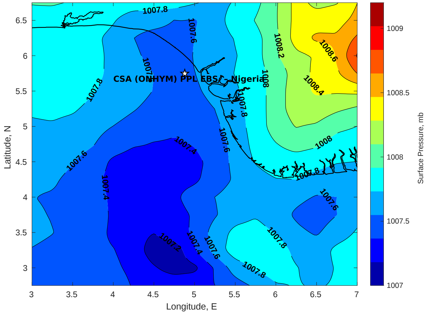
Surface Pressure (mb) for CSA (ONHYM) PPL EBS - Nigeria at 04-Mar-2025 06:00:00
